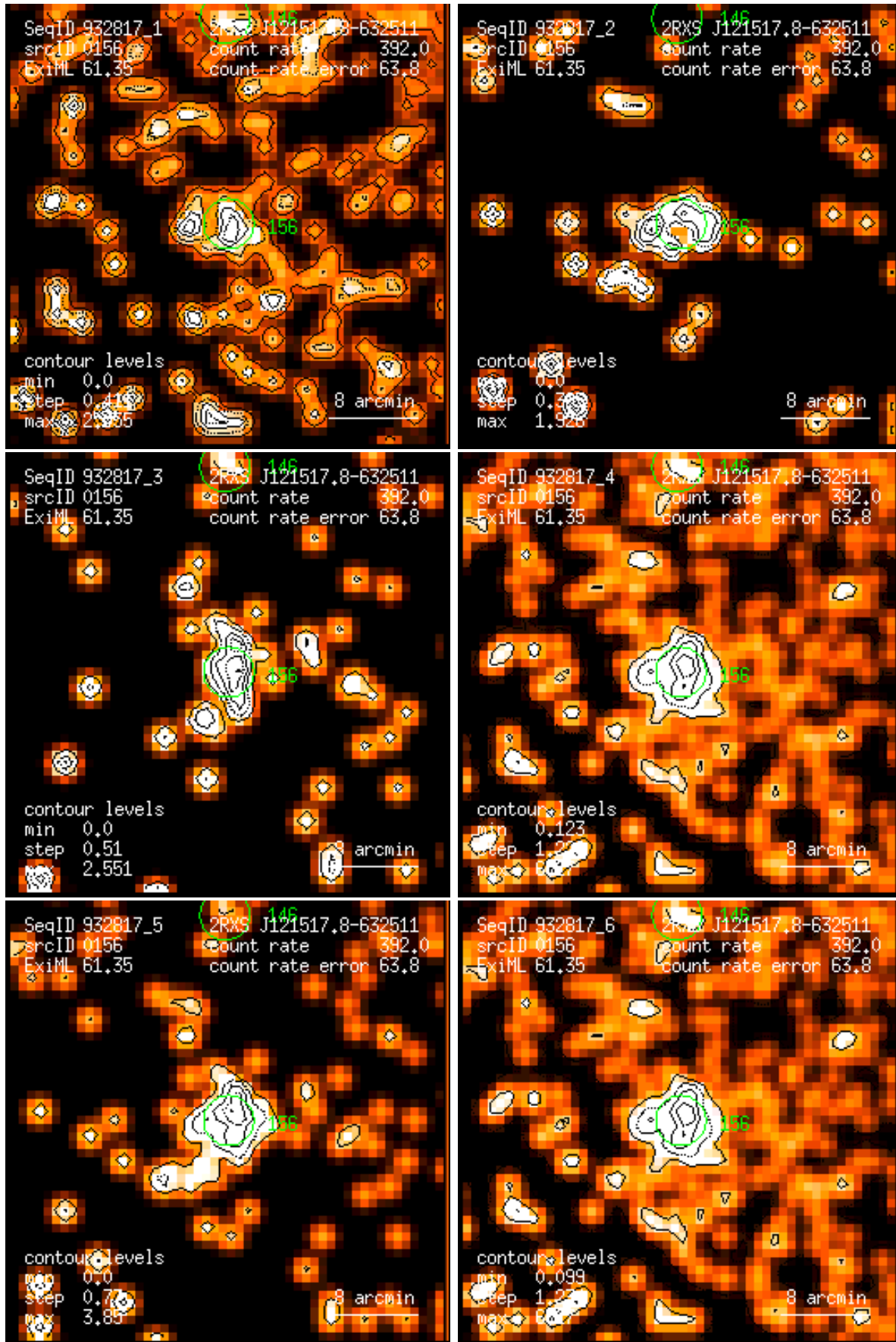
Figure 156: RASS 932817: detection 0156: band rate images, Gaussian filter: (1) PSPC channels 11 – 41, (2) 52 – 90, (3) 91 – 201, (4) 11 – 235, (5) 52 – 201, (6) 11 – 201. Broad band rates in counts/ks. Band rate contour levels in counts/ks/arcmin 2 .
