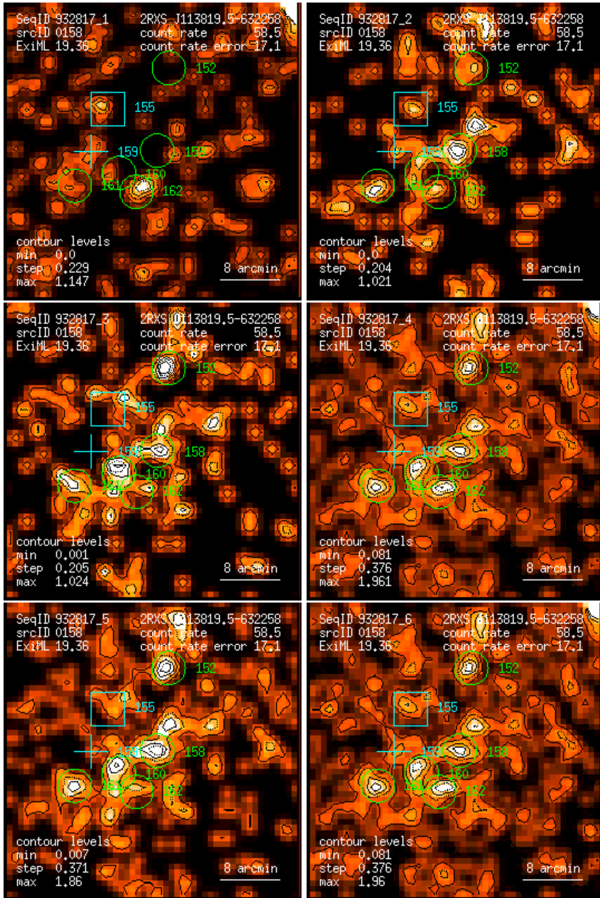
Figure 158: RASS 932817: detection 0158: band rate images, Gaussian filter: (1) PSPC channels 11 – 41, (2) 52 – 90, (3) 91 – 201, (4) 11 – 235, (5) 52 – 201, (6) 11 – 201. Broad band rates in counts/ks. Band rate contour levels in counts/ks/arcmin 2 .
