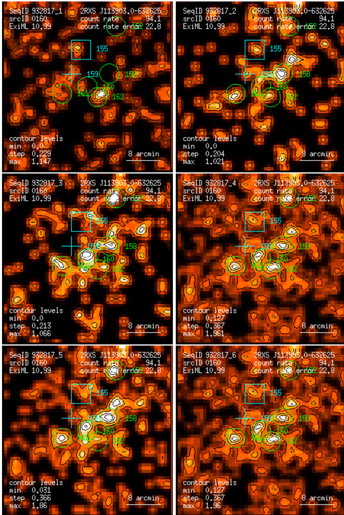
Figure 160: RASS 932817: detection 0160: band rate images, Gaussian filter: (1) PSPC channels 11 – 41, (2) 52 – 90, (3) 91 – 201, (4) 11 – 235, (5) 52 – 201, (6) 11 – 201. Broad band rates in counts/ks. Band rate contour levels in counts/ks/arcmin 2 .
