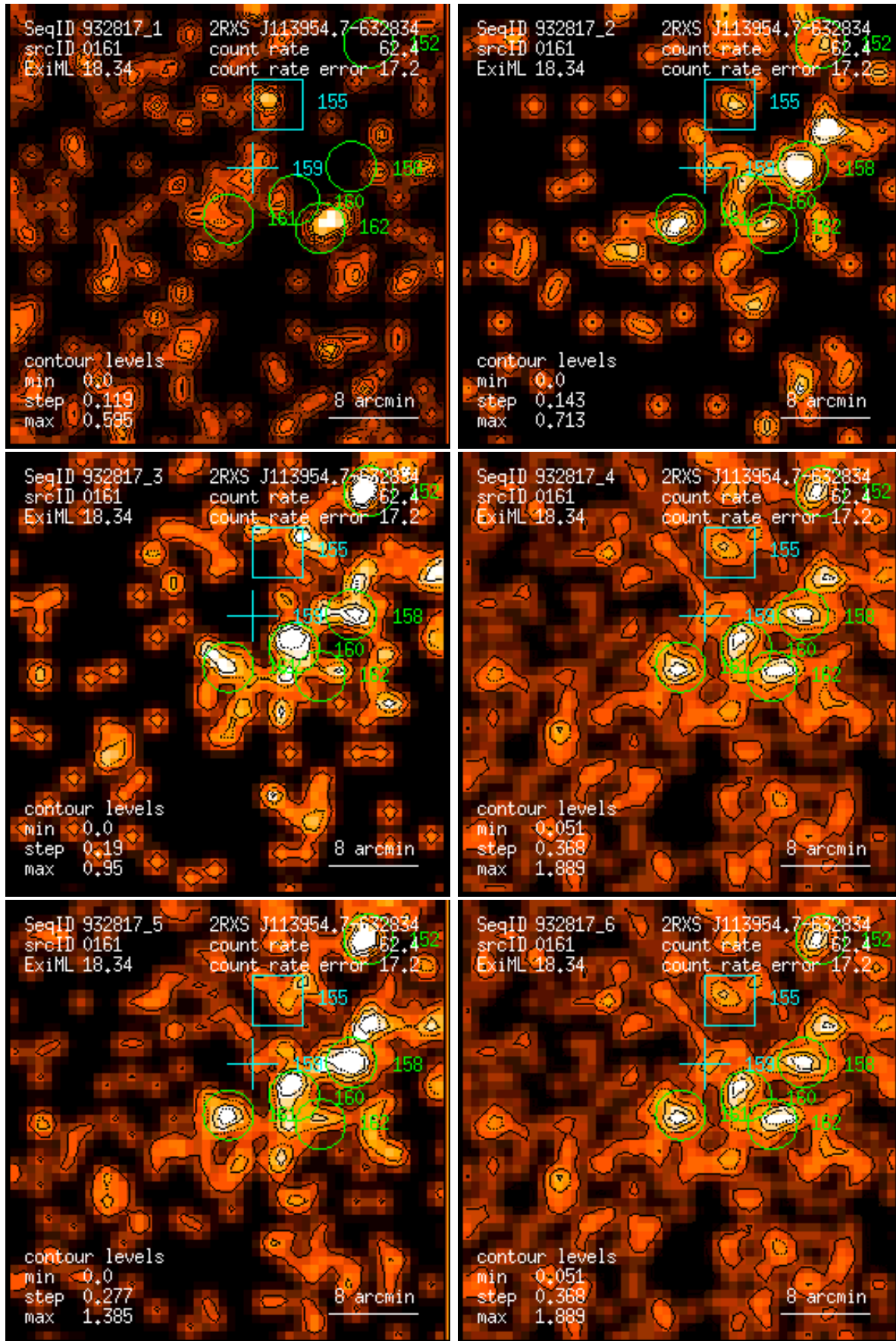
Figure 161: RASS 932817: detection 0161: band rate images, Gaussian filter: (1) PSPC channels 11 – 41, (2) 52 – 90, (3) 91 – 201, (4) 11 – 235, (5) 52 – 201, (6) 11 – 201. Broad band rates in counts/ks. Band rate contour levels in counts/ks/arcmin 2 .
