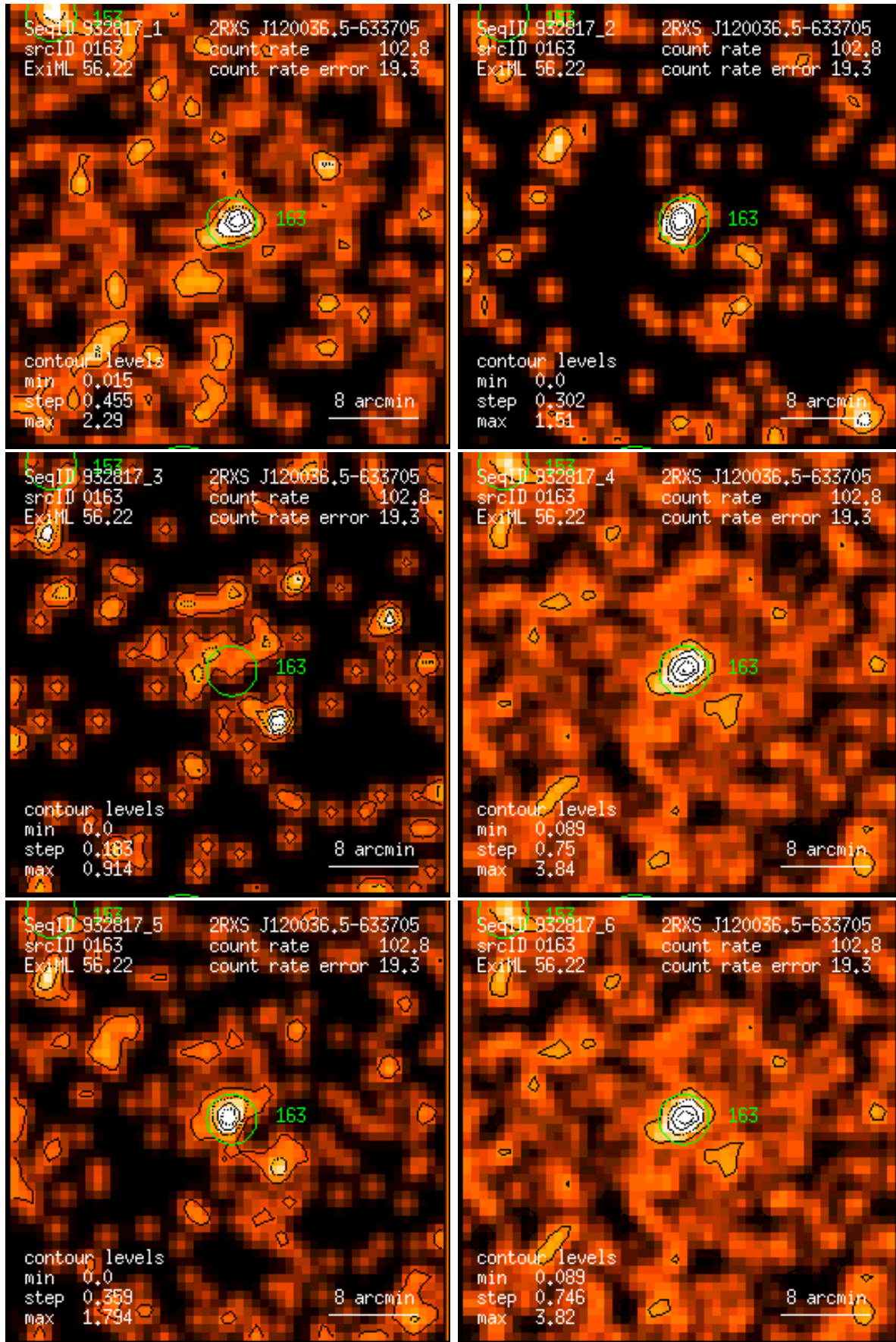
Figure 163: RASS 932817: detection 0163: band rate images, Gaussian filter: (1) PSPC channels 11 – 41, (2) 52 – 90, (3) 91 – 201, (4) 11 – 235, (5) 52 – 201, (6) 11 – 201. Broad band rates in counts/ks. Band rate contour levels in counts/ks/arcmin 2 .
