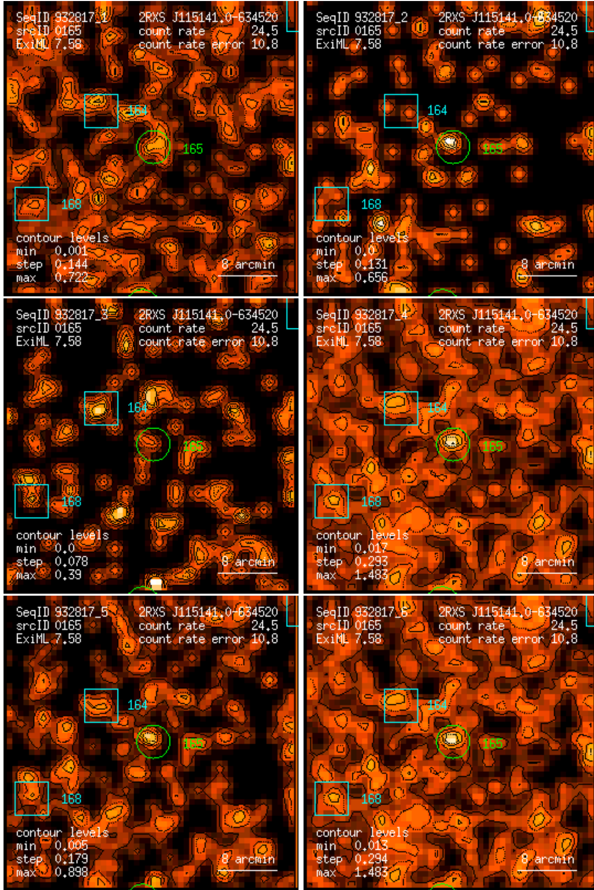
Figure 165: RASS 932817: detection 0165: band rate images, Gaussian filter: (1) PSPC channels 11 – 41, (2) 52 – 90, (3) 91 – 201, (4) 11 – 235, (5) 52 – 201, (6) 11 – 201. Broad band rates in counts/ks. Band rate contour levels in counts/ks/arcmin 2 .
