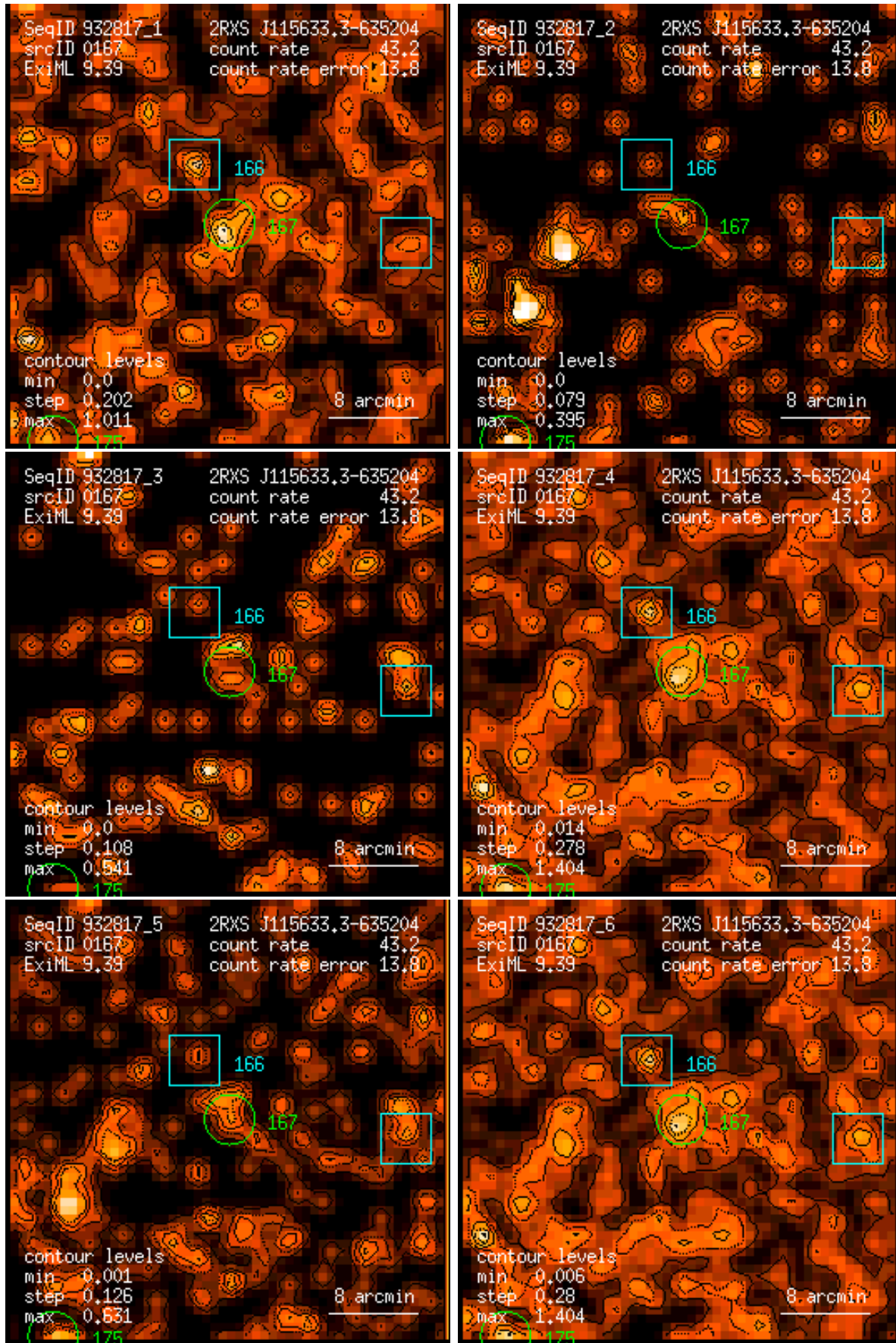
Figure 167: RASS 932817: detection 0167: band rate images, Gaussian filter: (1) PSPC channels 11 – 41, (2) 52 – 90, (3) 91 – 201, (4) 11 – 235, (5) 52 – 201, (6) 11 – 201. Broad band rates in counts/ks. Band rate contour levels in counts/ks/arcmin 2 .
