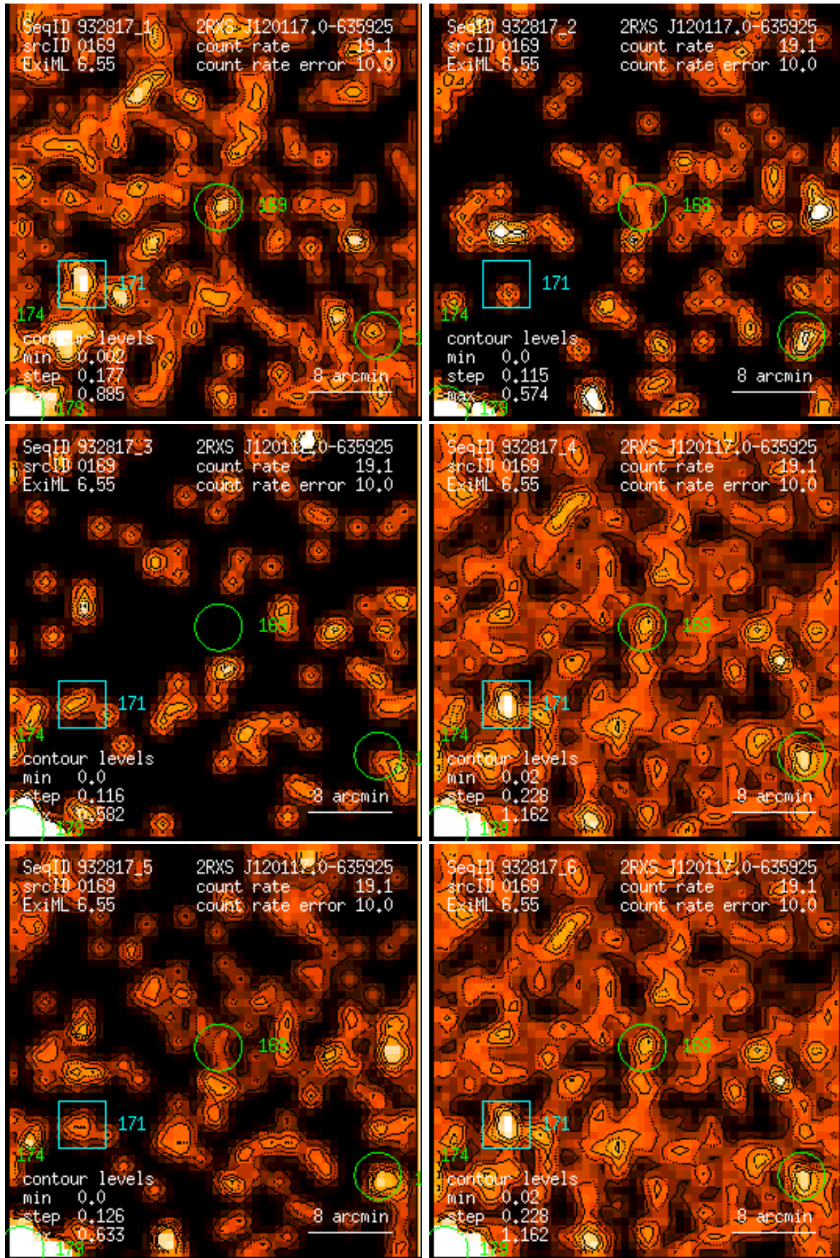
Figure 169: RASS 932817: detection 0169: band rate images, Gaussian filter: (1) PSPC channels 11 – 41, (2) 52 – 90, (3) 91 – 201, (4) 11 – 235, (5) 52 – 201, (6) 11 – 201. Broad band rates in counts/ks. Band rate contour levels in counts/ks/arcmin 2 .
