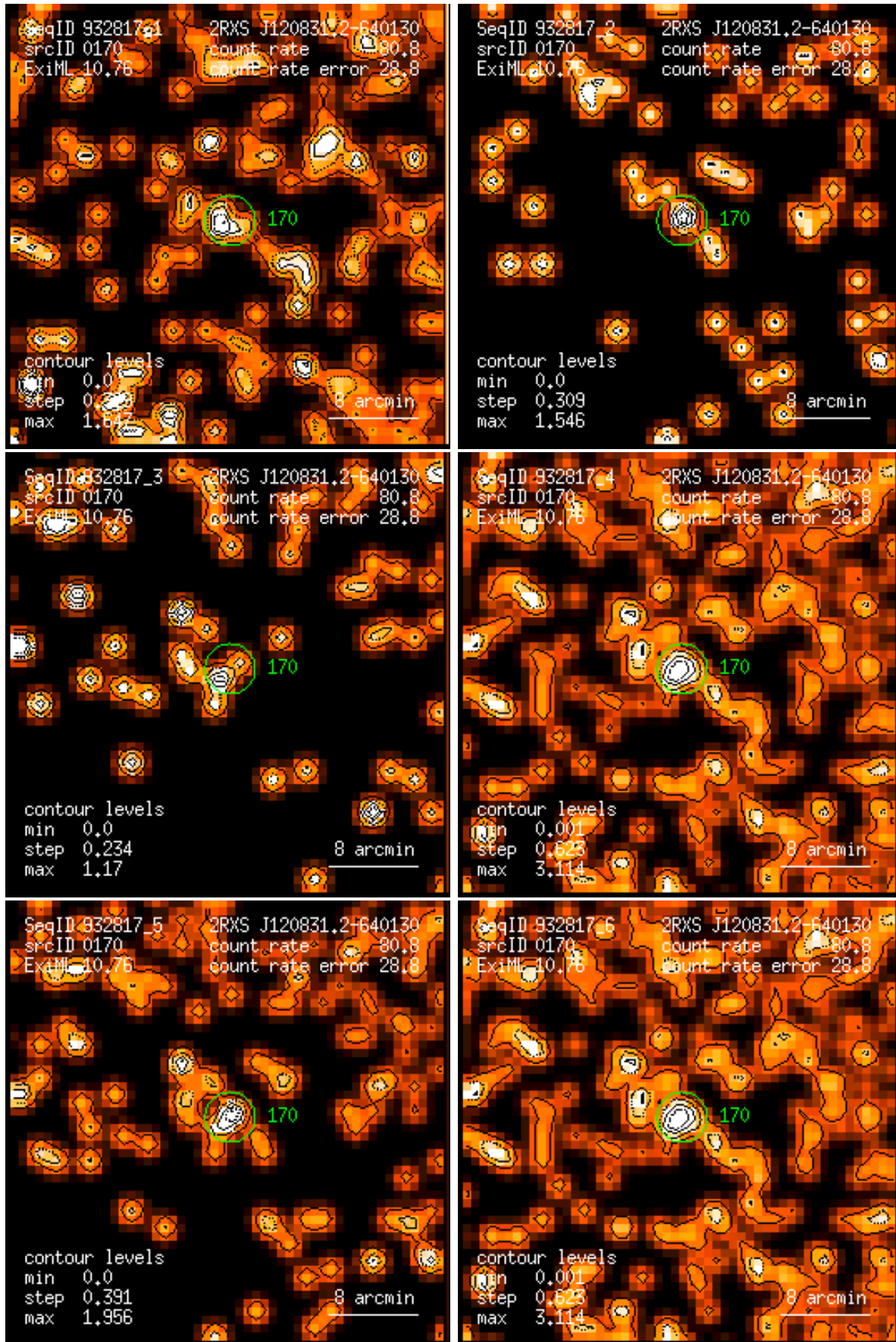
Figure 170: RASS 932817: detection 0170: band rate images, Gaussian filter: (1) PSPC channels 11 – 41, (2) 52 – 90, (3) 91 – 201, (4) 11 – 235, (5) 52 – 201, (6) 11 – 201. Broad band rates in counts/ks. Band rate contour levels in counts/ks/arcmin 2 .
