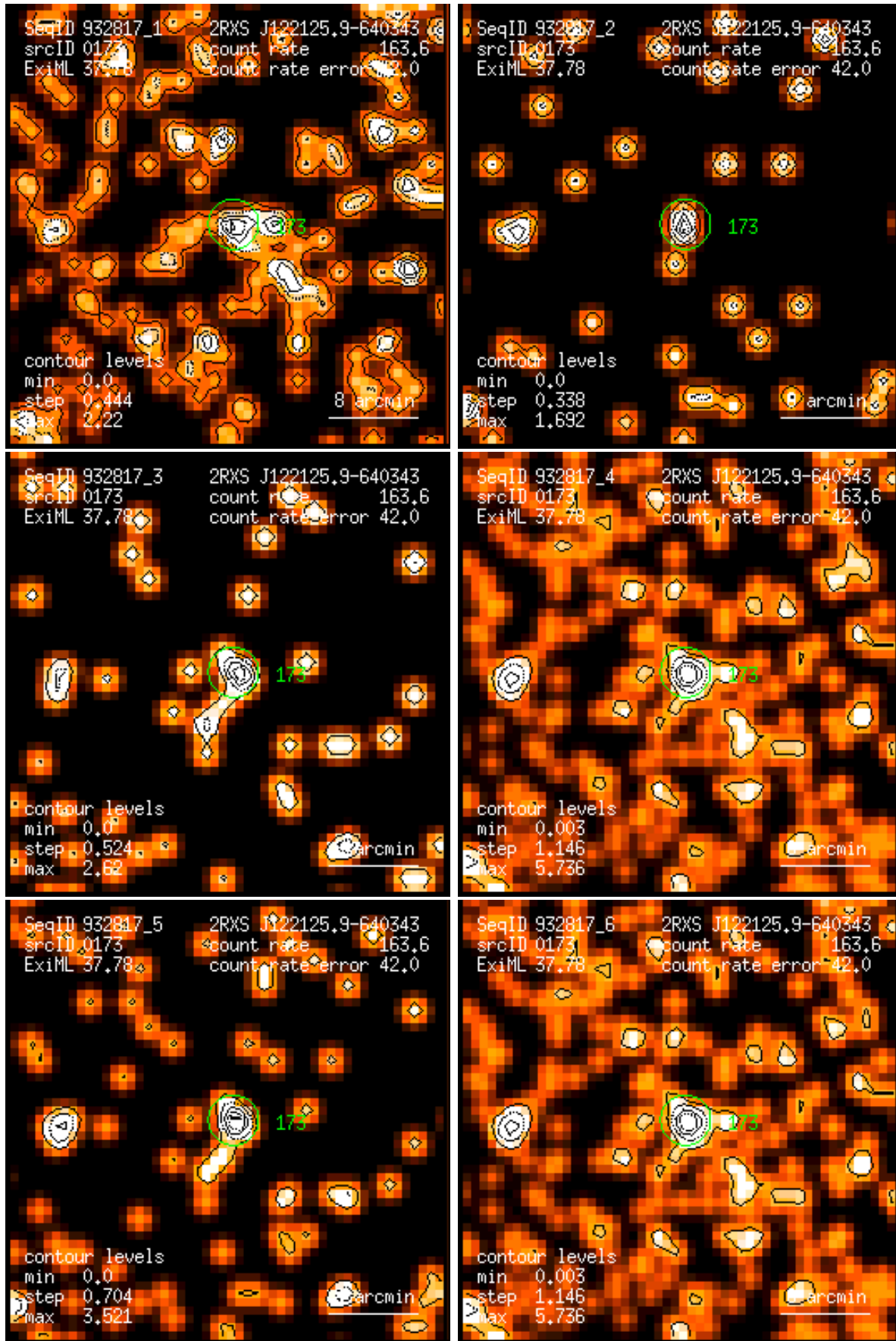
Figure 173: RASS 932817: detection 0173: band rate images, Gaussian filter: (1) PSPC channels 11 – 41, (2) 52 – 90, (3) 91 – 201, (4) 11 – 235, (5) 52 – 201, (6) 11 – 201. Broad band rates in counts/ks. Band rate contour levels in counts/ks/arcmin 2 .
