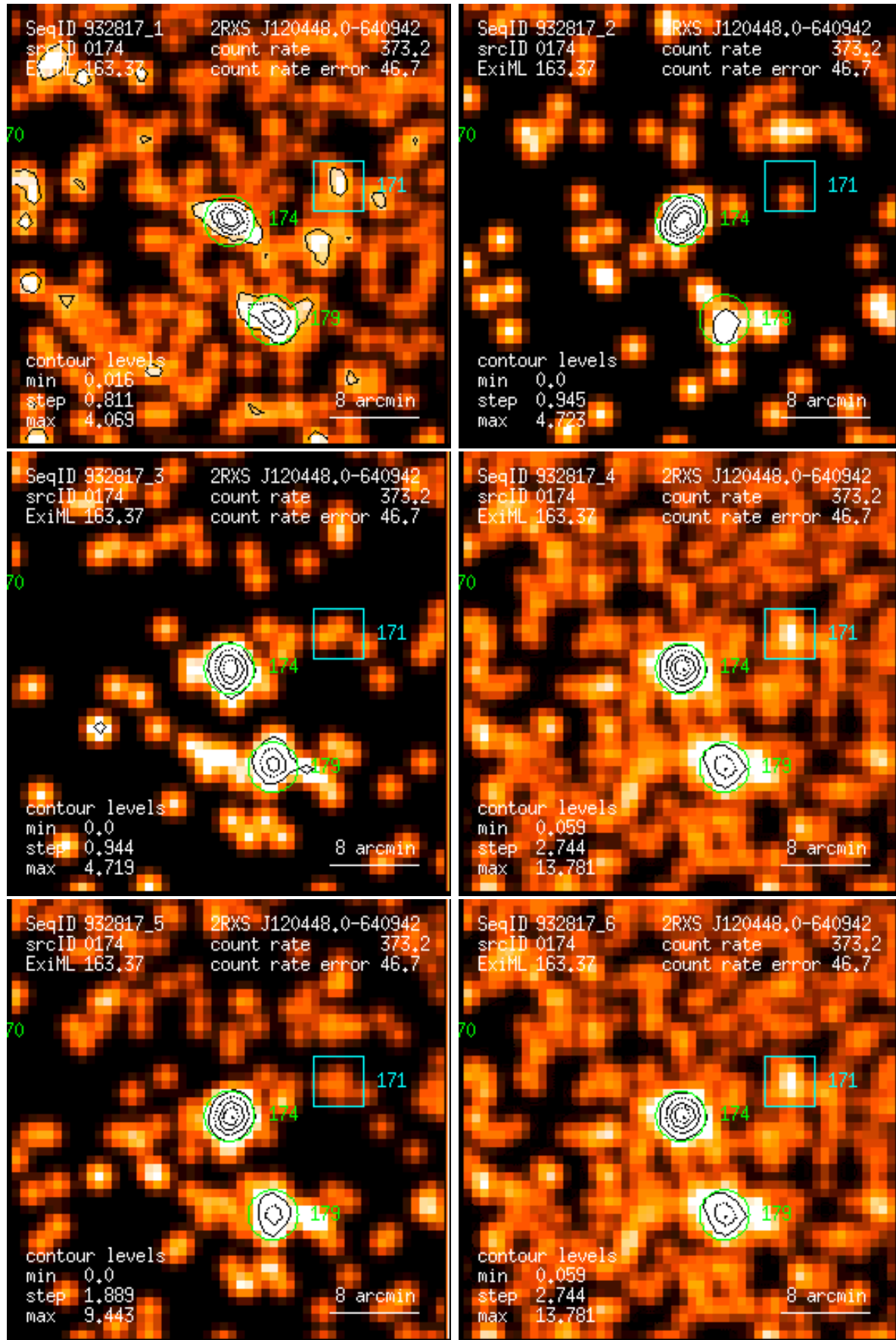
Figure 174: RASS 932817: detection 0174: band rate images, Gaussian filter: (1) PSPC channels 11 – 41, (2) 52 – 90, (3) 91 – 201, (4) 11 – 235, (5) 52 – 201, (6) 11 – 201. Broad band rates in counts/ks. Band rate contour levels in counts/ks/arcmin 2 .
