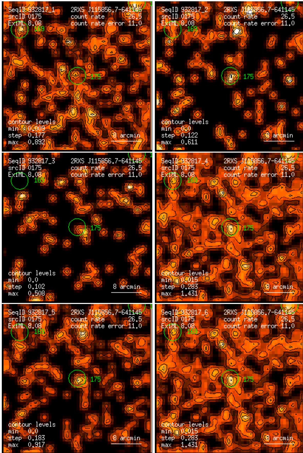
Figure 175: RASS 932817: detection 0175: band rate images, Gaussian filter: (1) PSPC channels 11 – 41, (2) 52 – 90, (3) 91 – 201, (4) 11 – 235, (5) 52 – 201, (6) 11 – 201. Broad band rates in counts/ks. Band rate contour levels in counts/ks/arcmin 2 .
