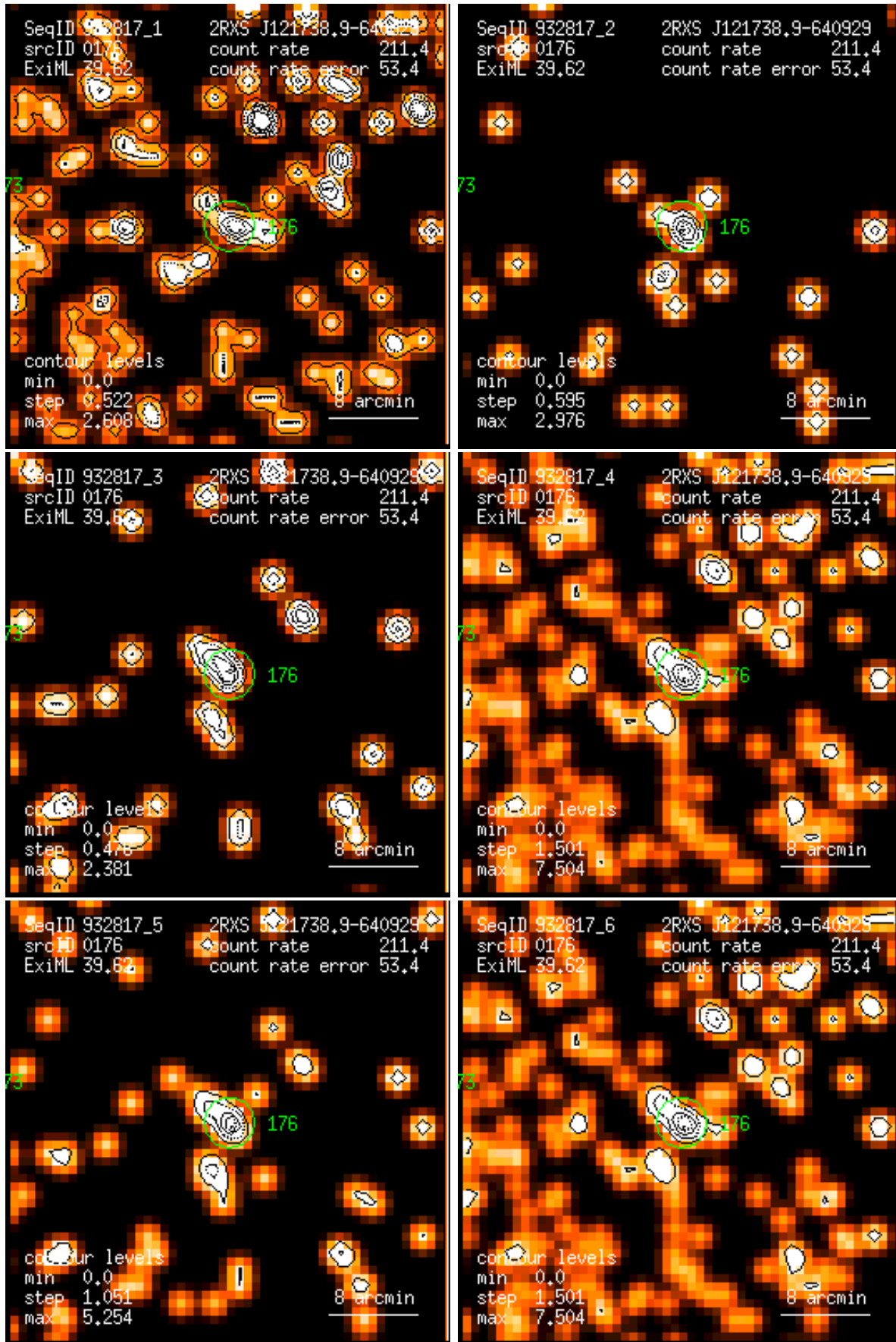
Figure 176: RASS 932817: detection 0176: band rate images, Gaussian filter: (1) PSPC channels 11 – 41, (2) 52 – 90, (3) 91 – 201, (4) 11 – 235, (5) 52 – 201, (6) 11 – 201. Broad band rates in counts/ks. Band rate contour levels in counts/ks/arcmin 2 .
