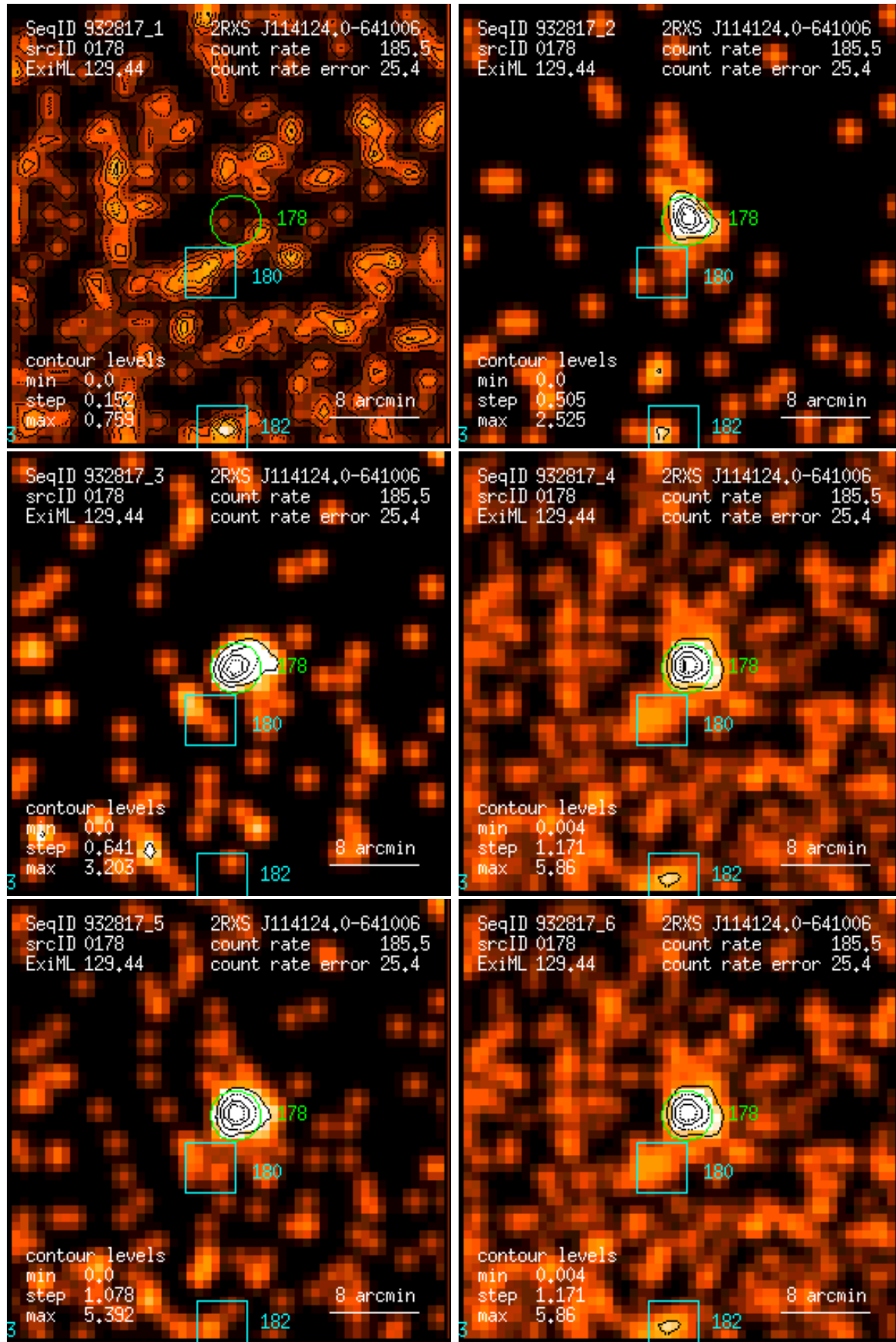
Figure 178: RASS 932817: detection 0178: band rate images, Gaussian filter: (1) PSPC channels 11 – 41, (2) 52 – 90, (3) 91 – 201, (4) 11 – 235, (5) 52 – 201, (6) 11 – 201. Broad band rates in counts/ks. Band rate contour levels in counts/ks/arcmin 2 .
