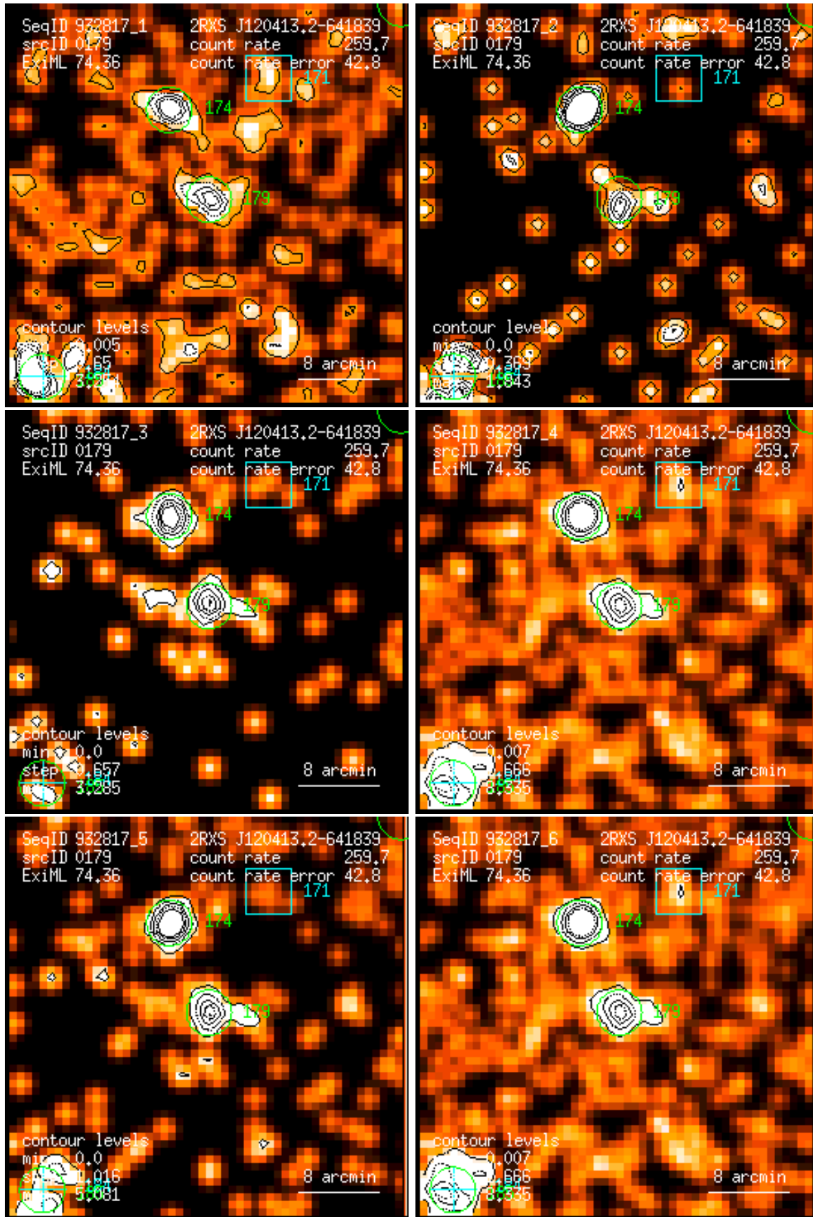
Figure 179: RASS 932817: detection 0179: band rate images, Gaussian filter: (1) PSPC channels 11 – 41, (2) 52 – 90, (3) 91 – 201, (4) 11 – 235, (5) 52 – 201, (6) 11 – 201. Broad band rates in counts/ks. Band rate contour levels in counts/ks/arcmin 2 .
