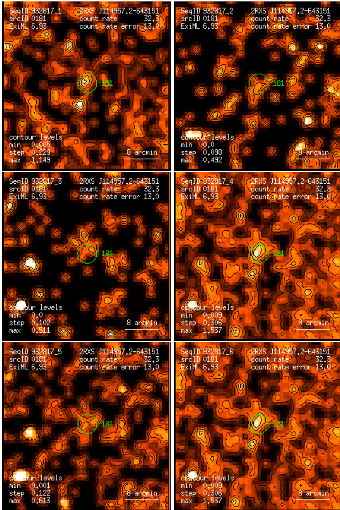
Figure 181: RASS 932817: detection 0181: band rate images, Gaussian filter: (1) PSPC channels 11 – 41, (2) 52 – 90, (3) 91 – 201, (4) 11 – 235, (5) 52 – 201, (6) 11 – 201. Broad band rates in counts/ks. Band rate contour levels in counts/ks/arcmin 2 .
