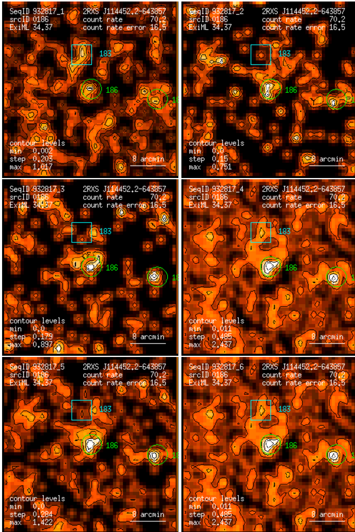
Figure 186: RASS 932817: detection 0186: band rate images, Gaussian filter: (1) PSPC channels 11 – 41, (2) 52 – 90, (3) 91 – 201, (4) 11 – 235, (5) 52 – 201, (6) 11 – 201. Broad band rates in counts/ks. Band rate contour levels in counts/ks/arcmin 2 .
