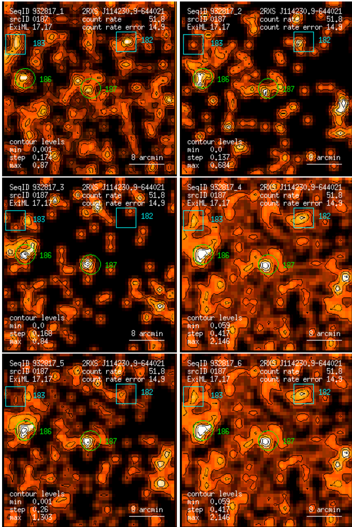
Figure 187: RASS 932817: detection 0187: band rate images, Gaussian filter: (1) PSPC channels 11 – 41, (2) 52 – 90, (3) 91 – 201, (4) 11 – 235, (5) 52 – 201, (6) 11 – 201. Broad band rates in counts/ks. Band rate contour levels in counts/ks/arcmin 2 .
