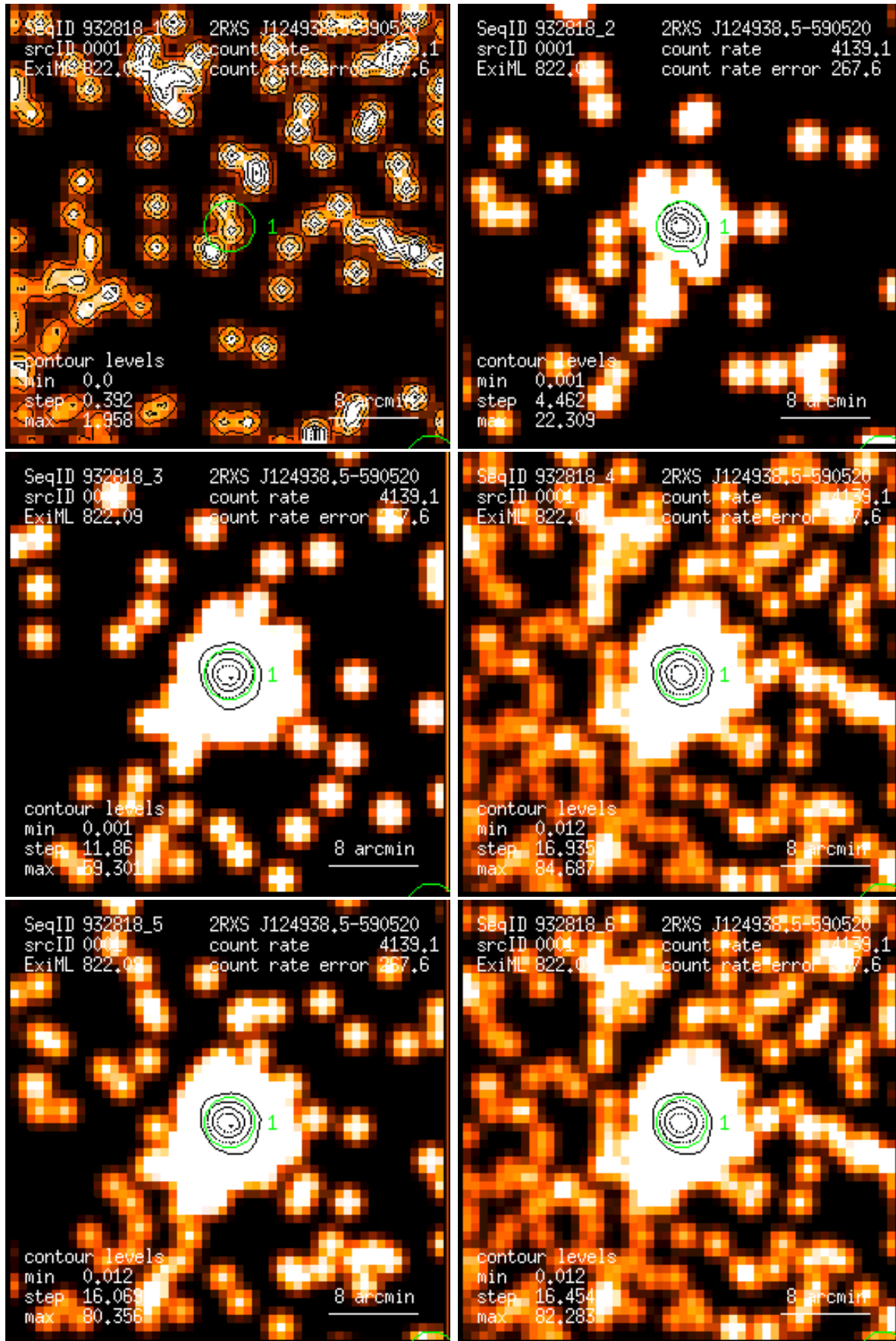
Figure 1: RASS 932818: detection 0001: band rate images, Gaussian filter: (1) PSPC channels 11 – 41, (2) 52 – 90, (3) 91 – 201, (4) 11 – 235, (5) 52 – 201, (6) 11 – 201. Broad band rates in counts/ks. Band rate contour levels in counts/ks/arcmin 2 .
