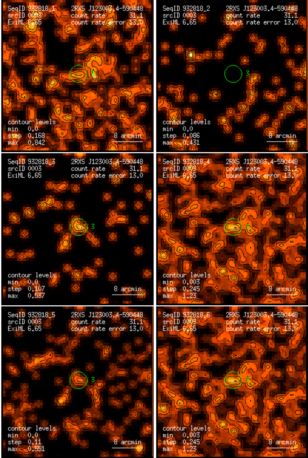
Figure 3: RASS 932818: detection 0003: band rate images, Gaussian filter: (1) PSPC channels 11 – 41, (2) 52 – 90, (3) 91 – 201, (4) 11 – 235, (5) 52 – 201, (6) 11 – 201. Broad band rates in counts/ks. Band rate contour levels in counts/ks/arcmin 2 .
