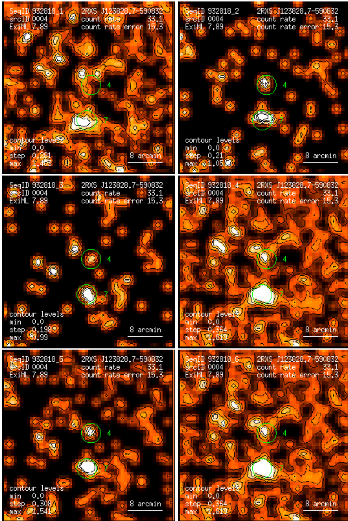
Figure 4: RASS 932818: detection 0004: band rate images, Gaussian filter: (1) PSPC channels 11 – 41, (2) 52 – 90, (3) 91 – 201, (4) 11 – 235, (5) 52 – 201, (6) 11 – 201. Broad band rates in counts/ks. Band rate contour levels in counts/ks/arcmin 2 .
