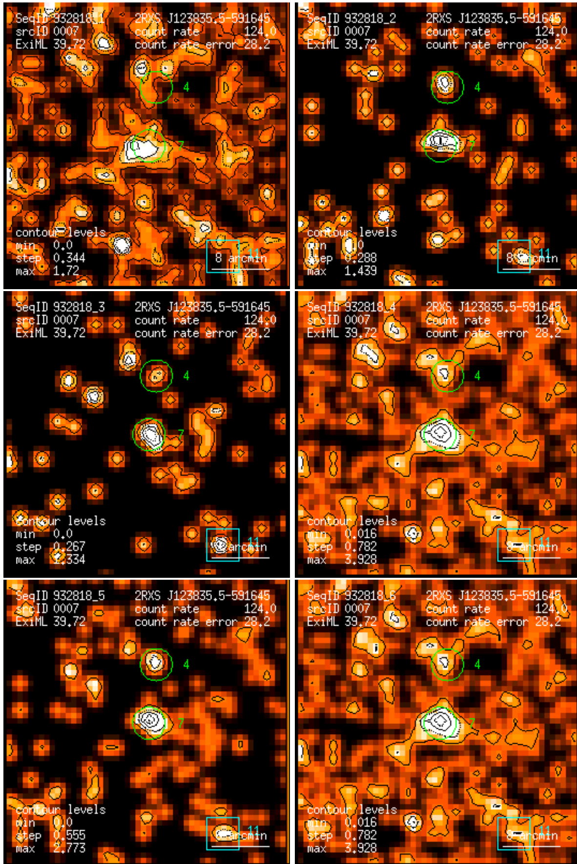
Figure 7: RASS 932818: detection 0007: band rate images, Gaussian filter: (1) PSPC channels 11 – 41, (2) 52 – 90, (3) 91 – 201, (4) 11 – 235, (5) 52 – 201, (6) 11 – 201. Broad band rates in counts/ks. Band rate contour levels in counts/ks/arcmin 2 .
