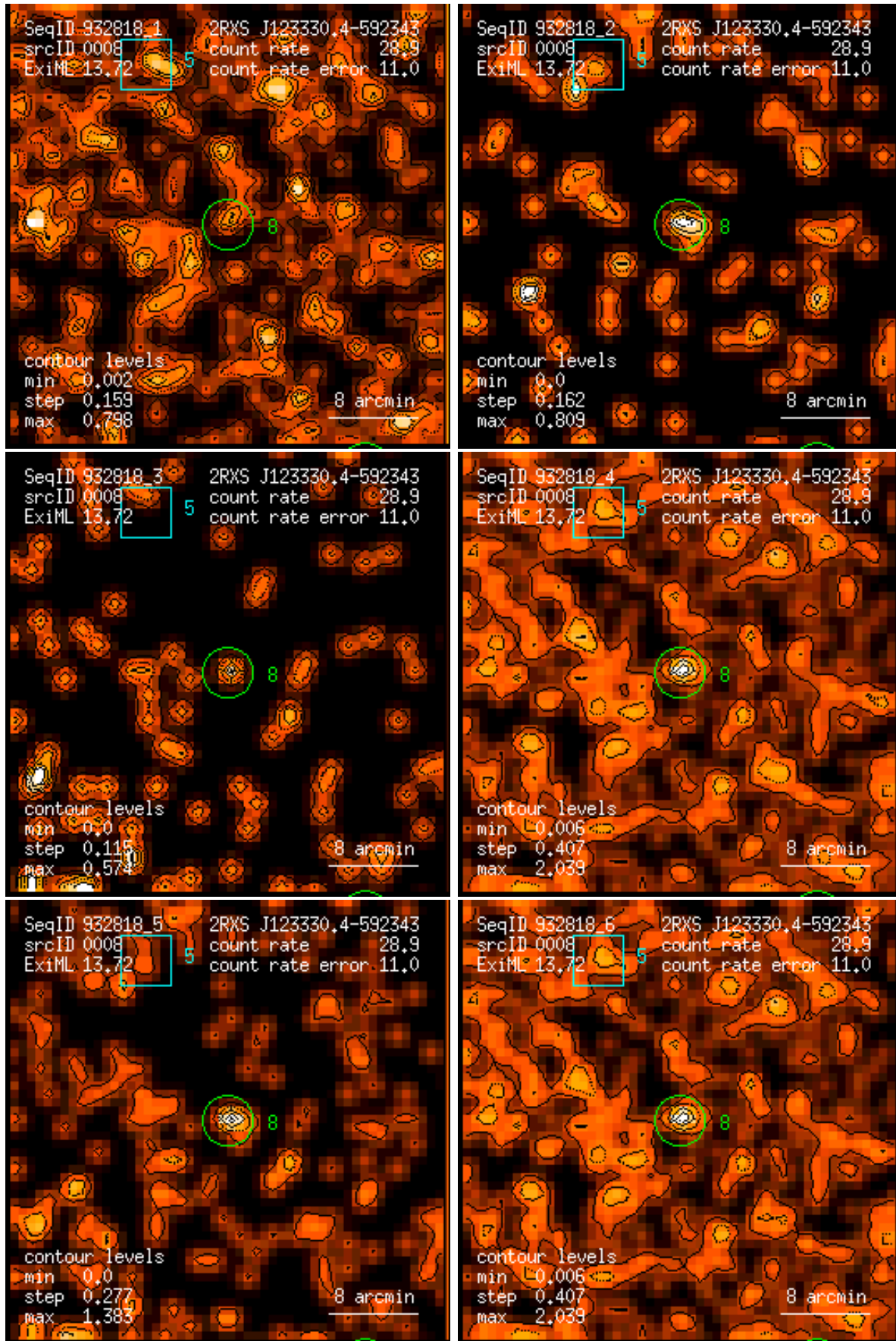
Figure 8: RASS 932818: detection 0008: band rate images, Gaussian filter: (1) PSPC channels 11 – 41, (2) 52 – 90, (3) 91 – 201, (4) 11 – 235, (5) 52 – 201, (6) 11 – 201. Broad band rates in counts/ks. Band rate contour levels in counts/ks/arcmin 2 .
