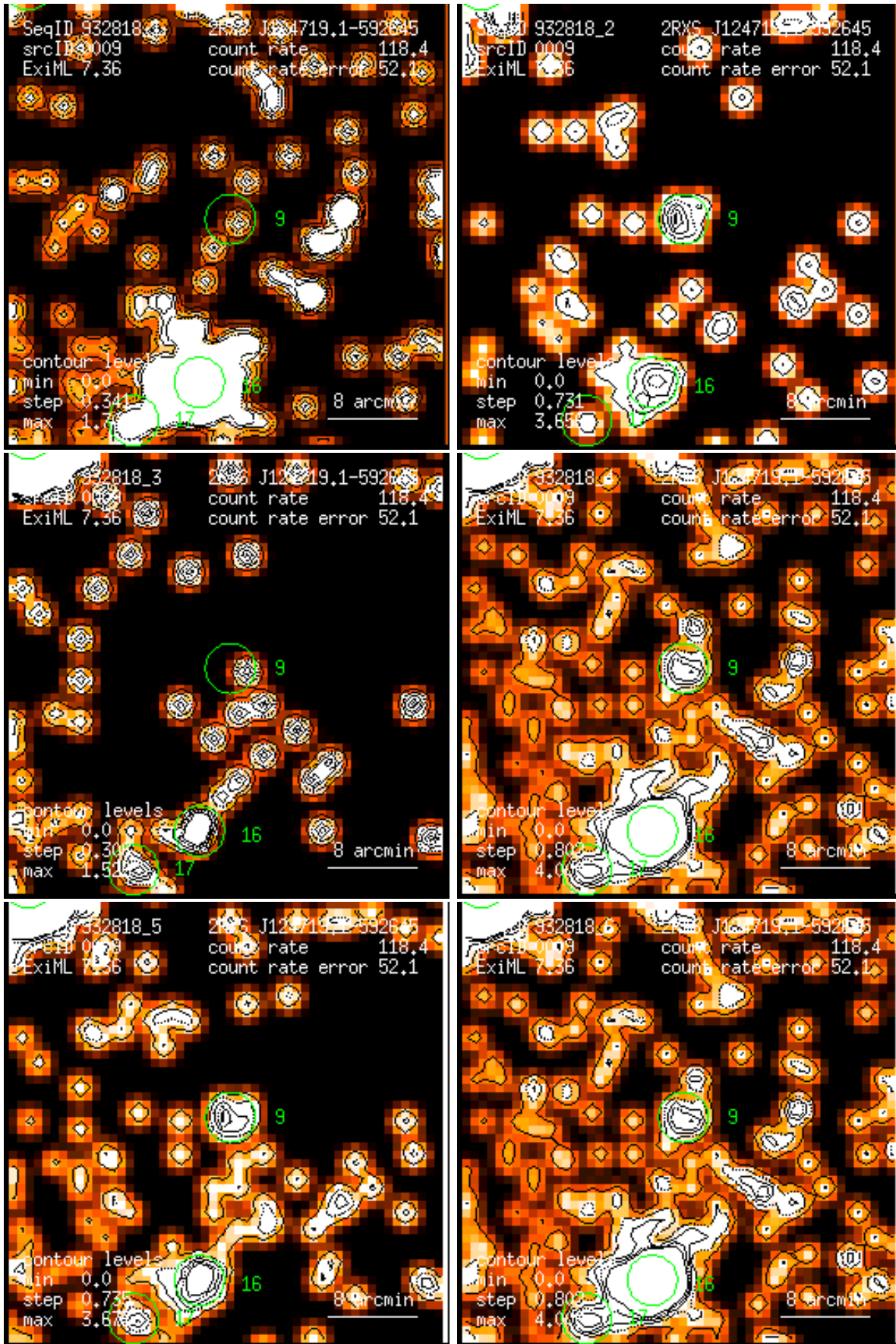
Figure 9: RASS 932818: detection 0009: band rate images, Gaussian filter: (1) PSPC channels 11 – 41, (2) 52 – 90, (3) 91 – 201, (4) 11 – 235, (5) 52 – 201, (6) 11 – 201. Broad band rates in counts/ks. Band rate contour levels in counts/ks/arcmin 2 .
