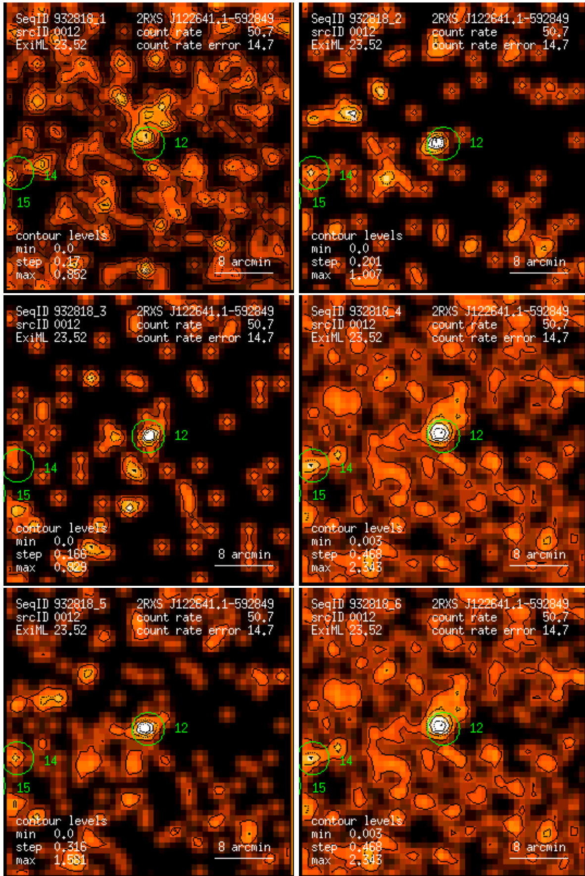
Figure 12: RASS 932818: detection 0012: band rate images, Gaussian filter: (1) PSPC channels 11 – 41, (2) 52 – 90, (3) 91 – 201, (4) 11 – 235, (5) 52 – 201, (6) 11 – 201. Broad band rates in counts/ks. Band rate contour levels in counts/ks/arcmin 2 .
