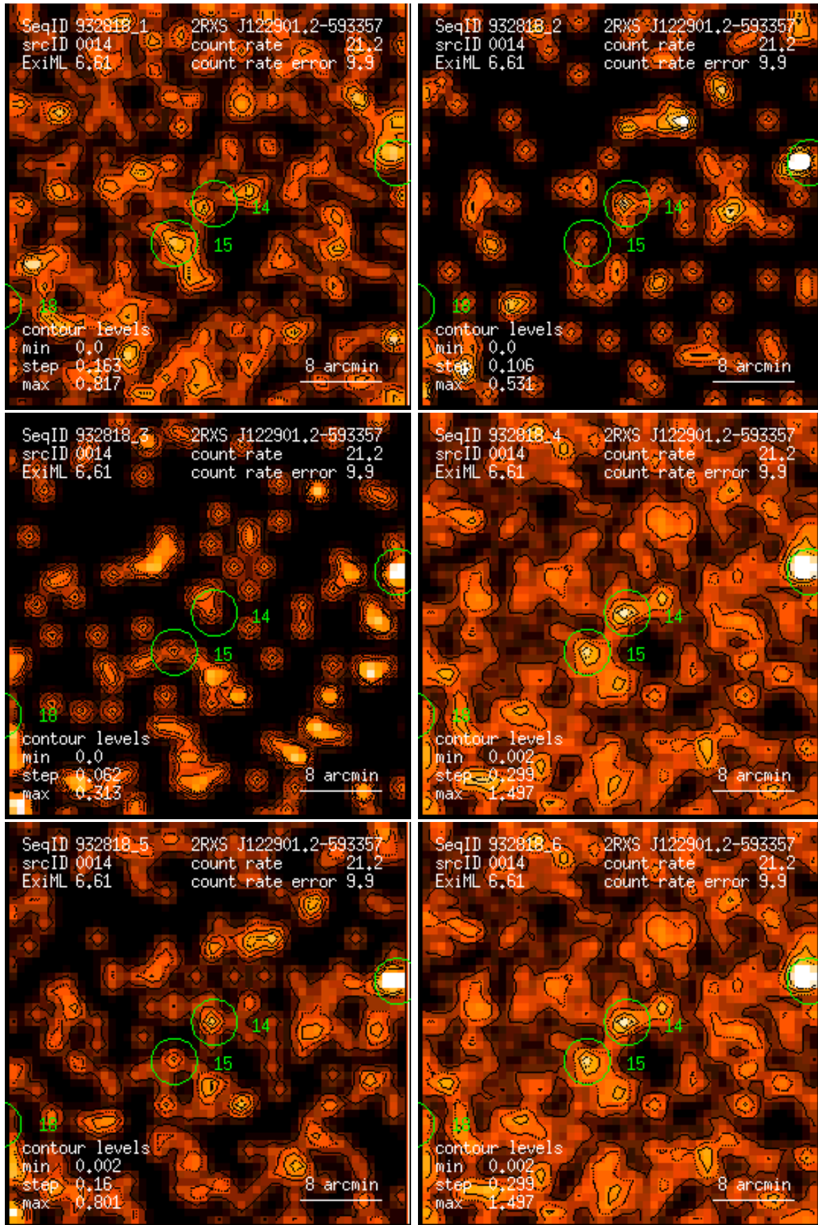
Figure 14: RASS 932818: detection 0014: band rate images, Gaussian filter: (1) PSPC channels 11 – 41, (2) 52 – 90, (3) 91 – 201, (4) 11 – 235, (5) 52 – 201, (6) 11 – 201. Broad band rates in counts/ks. Band rate contour levels in counts/ks/arcmin 2 .
