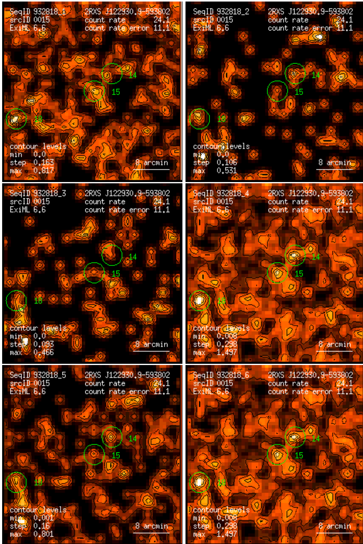
Figure 15: RASS 932818: detection 0015: band rate images, Gaussian filter: (1) PSPC channels 11 – 41, (2) 52 – 90, (3) 91 – 201, (4) 11 – 235, (5) 52 – 201, (6) 11 – 201. Broad band rates in counts/ks. Band rate contour levels in counts/ks/arcmin 2 .
