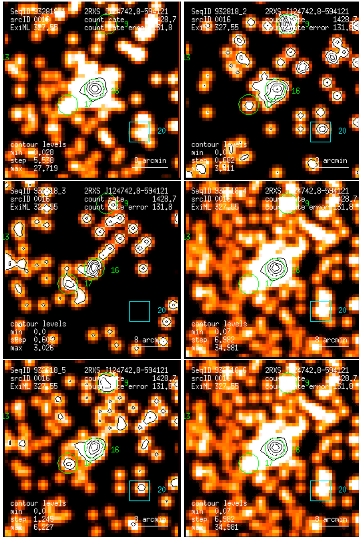
Figure 16: RASS 932818: detection 0016: band rate images, Gaussian filter: (1) PSPC channels 11 – 41, (2) 52 – 90, (3) 91 – 201, (4) 11 – 235, (5) 52 – 201, (6) 11 – 201. Broad band rates in counts/ks. Band rate contour levels in counts/ks/arcmin 2 .
