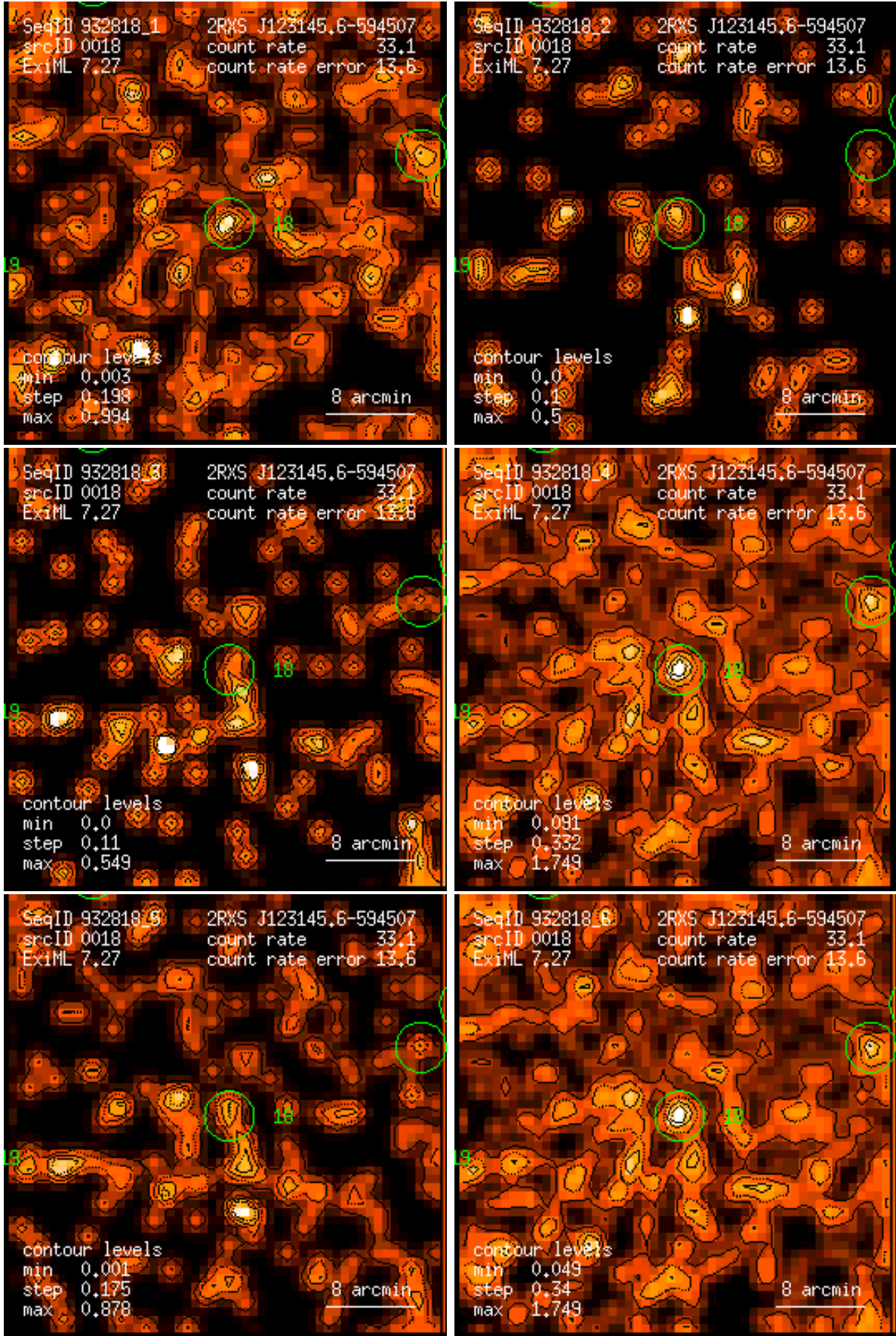
Figure 18: RASS 932818: detection 0018: band rate images, Gaussian filter: (1) PSPC channels 11 – 41, (2) 52 – 90, (3) 91 – 201, (4) 11 – 235, (5) 52 – 201, (6) 11 – 201. Broad band rates in counts/ks. Band rate contour levels in counts/ks/arcmin 2 .
