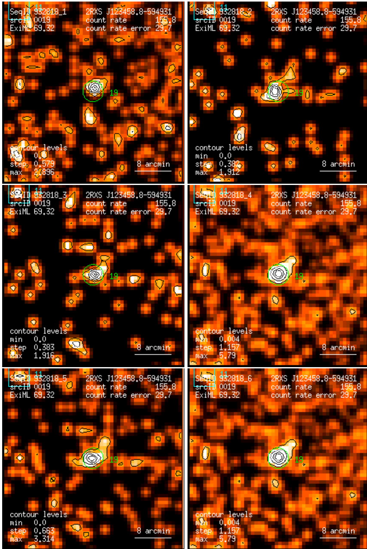
Figure 19: RASS 932818: detection 0019: band rate images, Gaussian filter: (1) PSPC channels 11 – 41, (2) 52 – 90, (3) 91 – 201, (4) 11 – 235, (5) 52 – 201, (6) 11 – 201. Broad band rates in counts/ks. Band rate contour levels in counts/ks/arcmin 2 .
