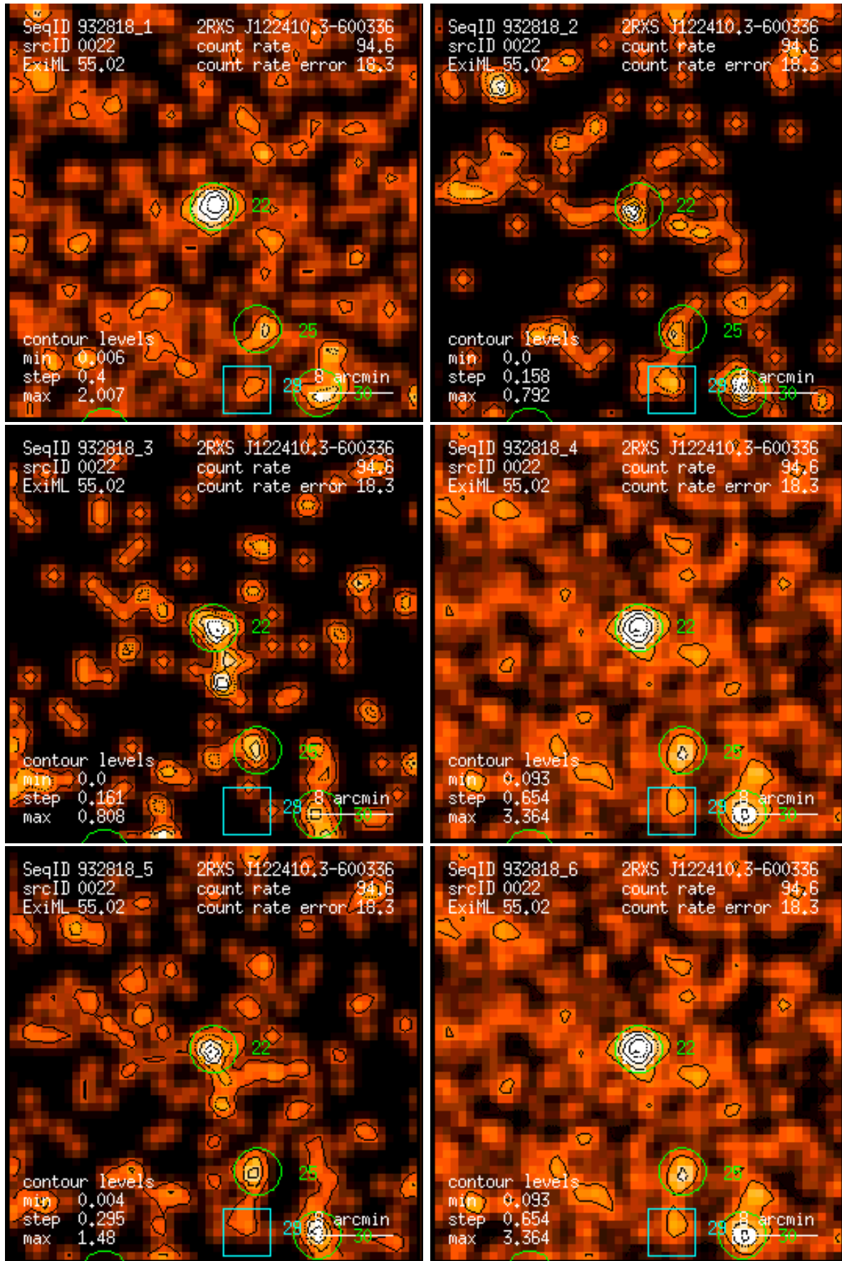
Figure 22: RASS 932818: detection 0022: band rate images, Gaussian filter: (1) PSPC channels 11 – 41, (2) 52 – 90, (3) 91 – 201, (4) 11 – 235, (5) 52 – 201, (6) 11 – 201. Broad band rates in counts/ks. Band rate contour levels in counts/ks/arcmin 2 .
