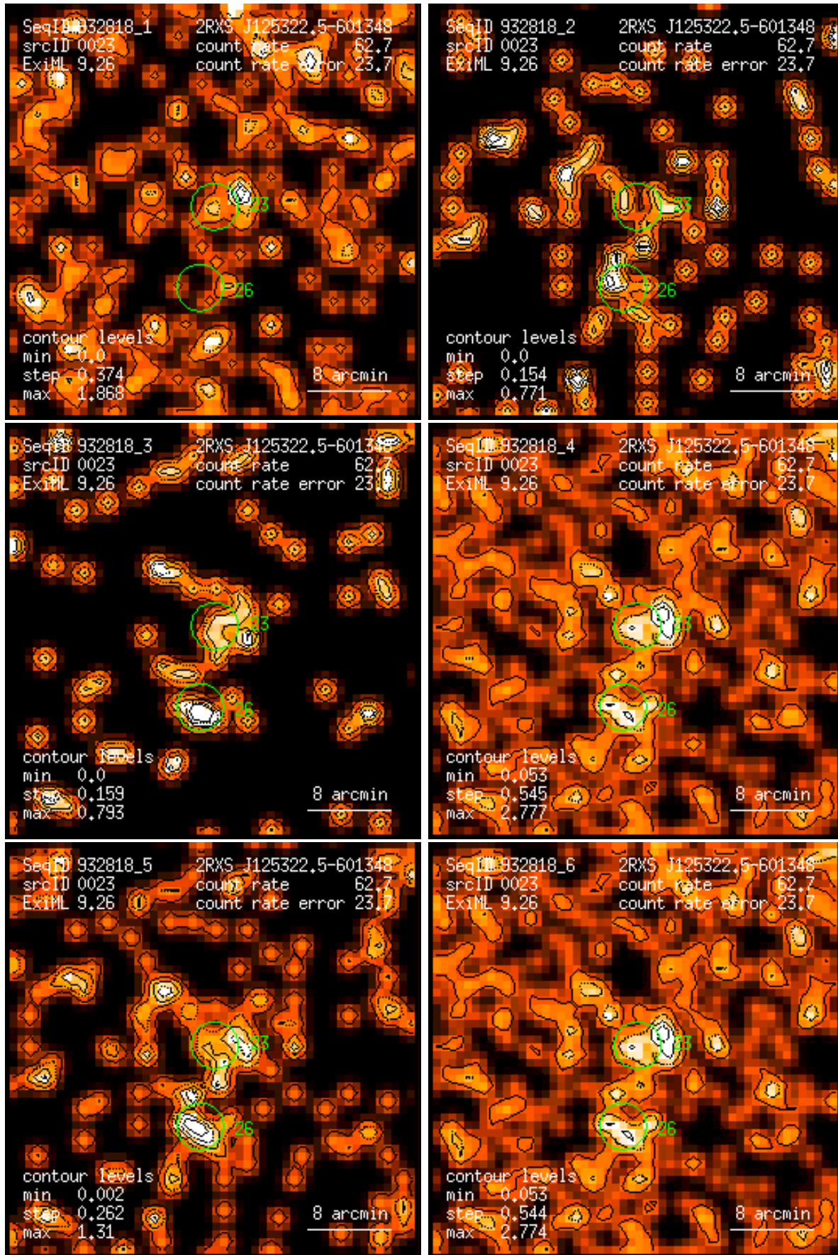
Figure 23: RASS 932818: detection 0023: band rate images, Gaussian filter: (1) PSPC channels 11 – 41, (2) 52 – 90, (3) 91 – 201, (4) 11 – 235, (5) 52 – 201, (6) 11 – 201. Broad band rates in counts/ks. Band rate contour levels in counts/ks/arcmin 2 .
