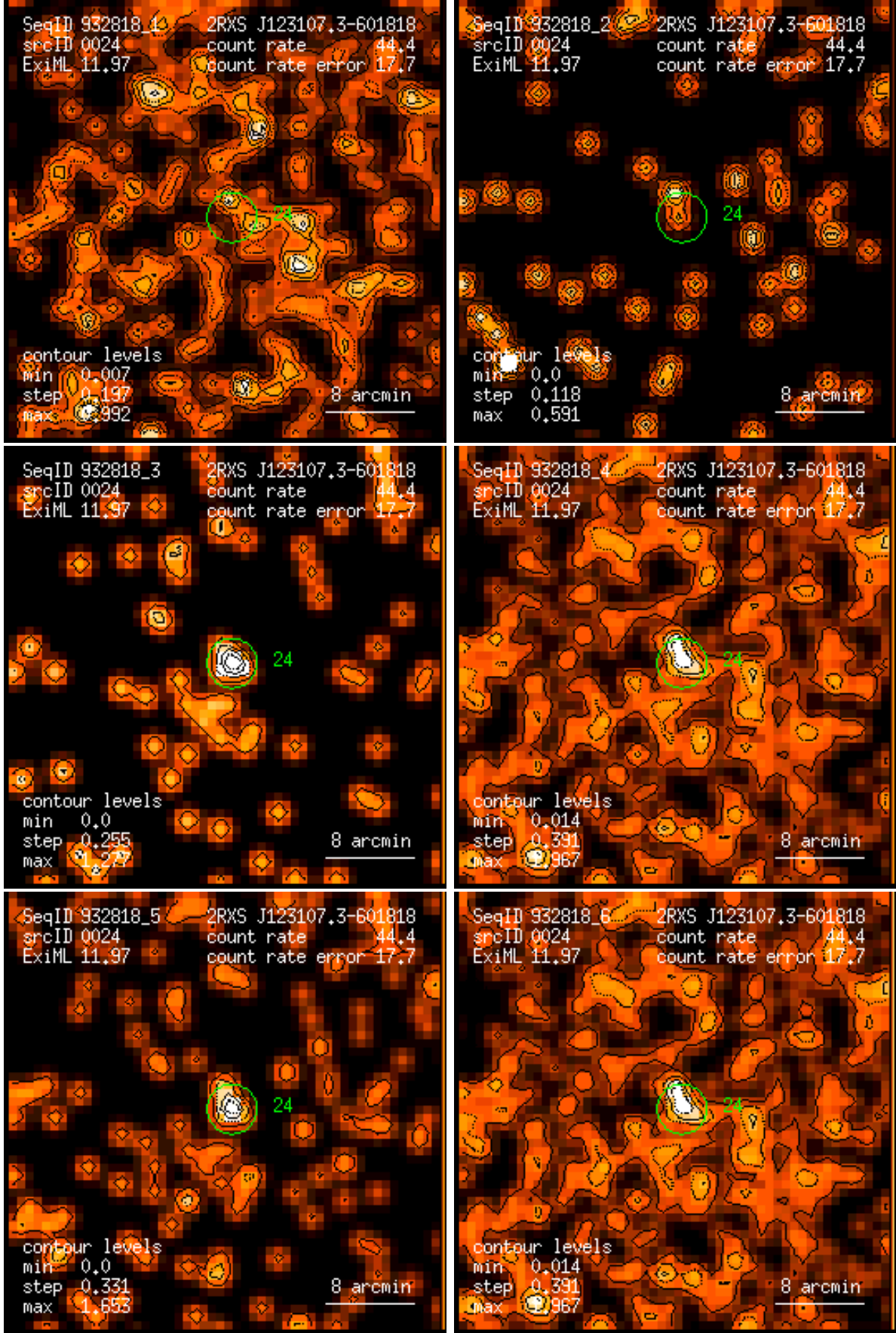
Figure 24: RASS 932818: detection 0024: band rate images, Gaussian filter: (1) PSPC channels 11 – 41, (2) 52 – 90, (3) 91 – 201, (4) 11 – 235, (5) 52 – 201, (6) 11 – 201. Broad band rates in counts/ks. Band rate contour levels in counts/ks/arcmin 2 .
