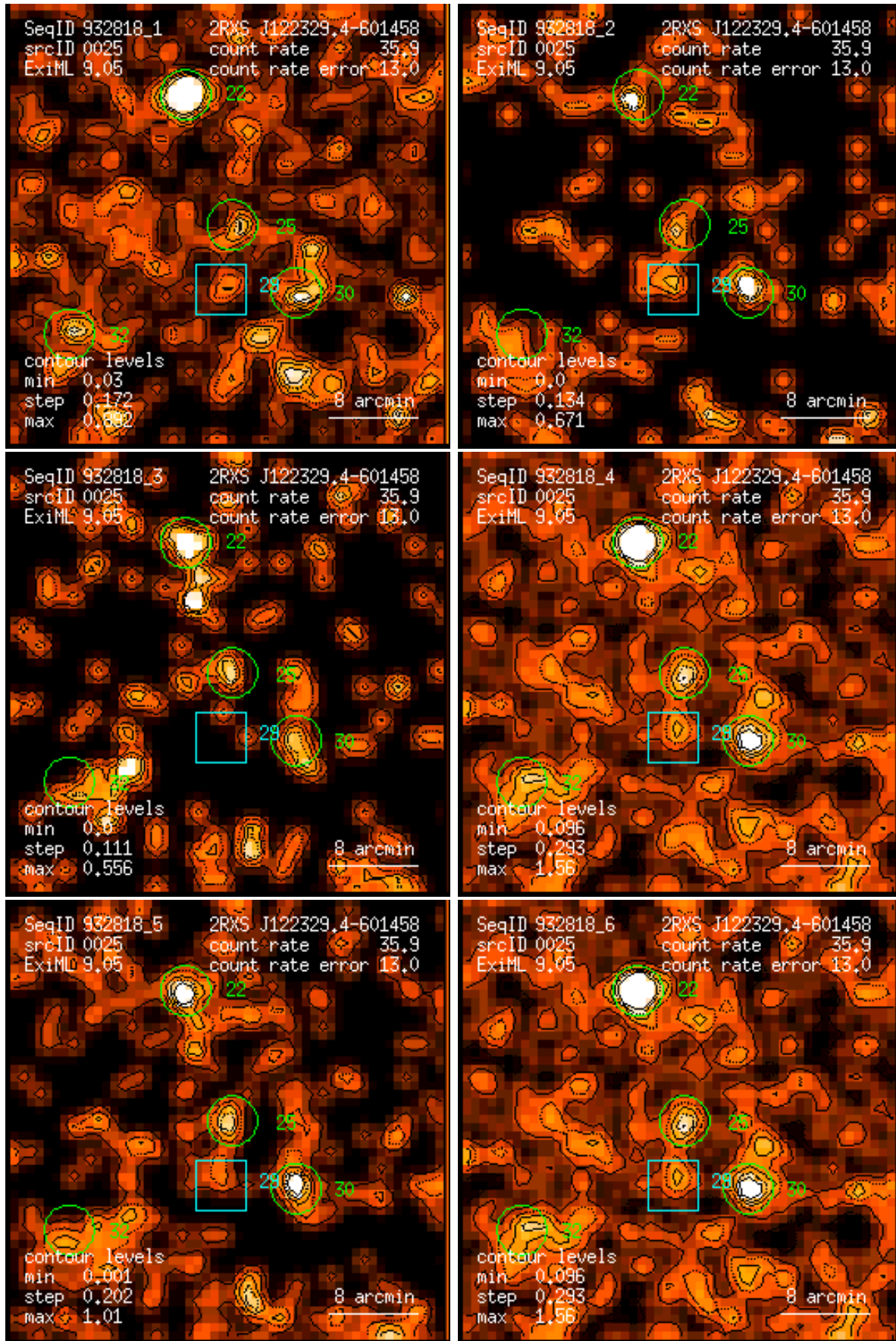
Figure 25: RASS 932818: detection 0025: band rate images, Gaussian filter: (1) PSPC channels 11 – 41, (2) 52 – 90, (3) 91 – 201, (4) 11 – 235, (5) 52 – 201, (6) 11 – 201. Broad band rates in counts/ks. Band rate contour levels in counts/ks/arcmin 2 .
