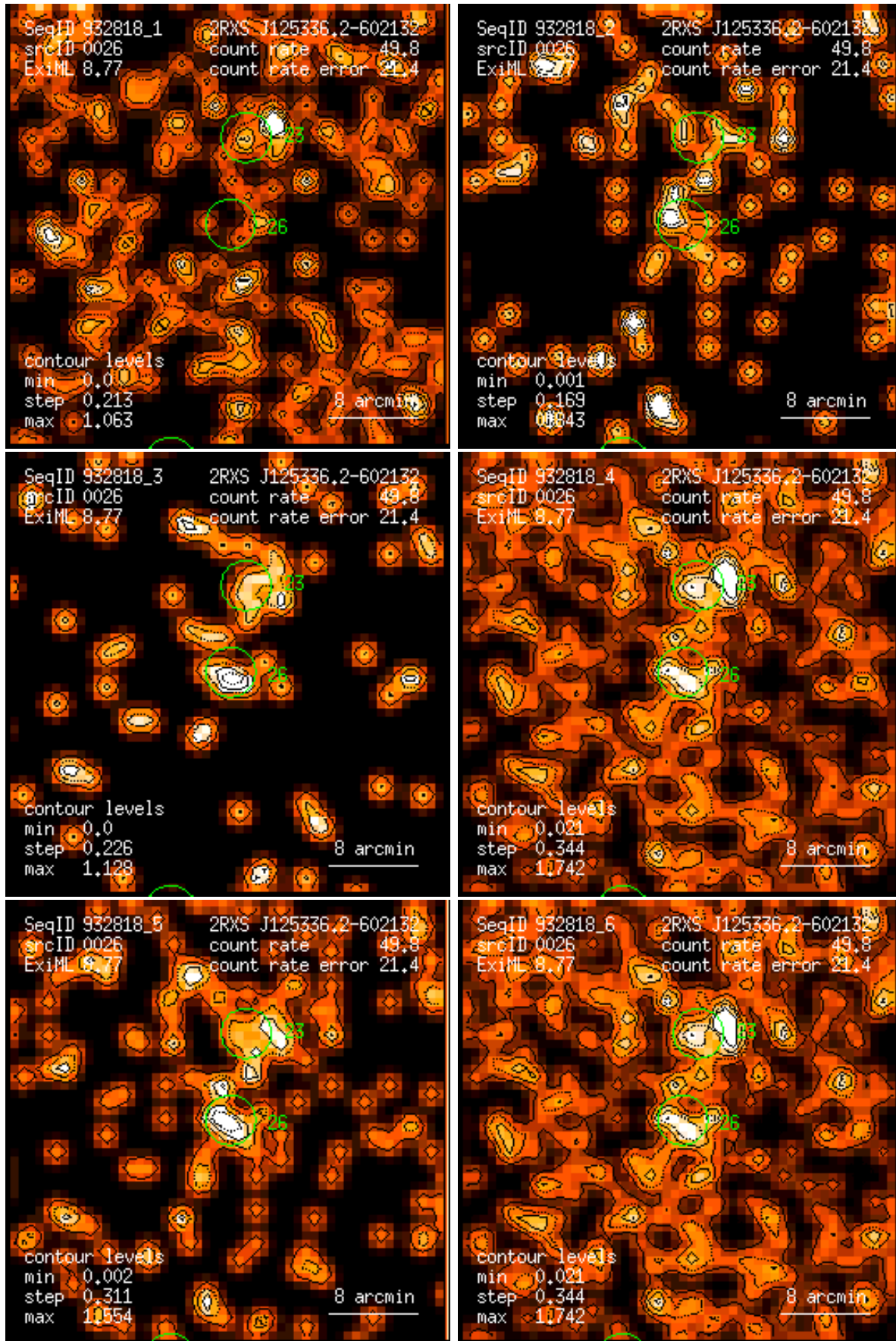
Figure 26: RASS 932818: detection 0026: band rate images, Gaussian filter: (1) PSPC channels 11 – 41, (2) 52 – 90, (3) 91 – 201, (4) 11 – 235, (5) 52 – 201, (6) 11 – 201. Broad band rates in counts/ks. Band rate contour levels in counts/ks/arcmin 2 .
