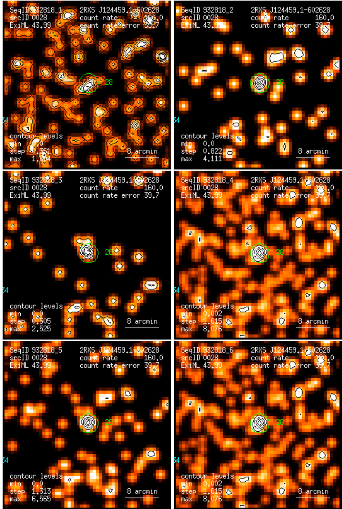
Figure 28: RASS 932818: detection 0028: band rate images, Gaussian filter: (1) PSPC channels 11 – 41, (2) 52 – 90, (3) 91 – 201, (4) 11 – 235, (5) 52 – 201, (6) 11 – 201. Broad band rates in counts/ks. Band rate contour levels in counts/ks/arcmin 2 .
