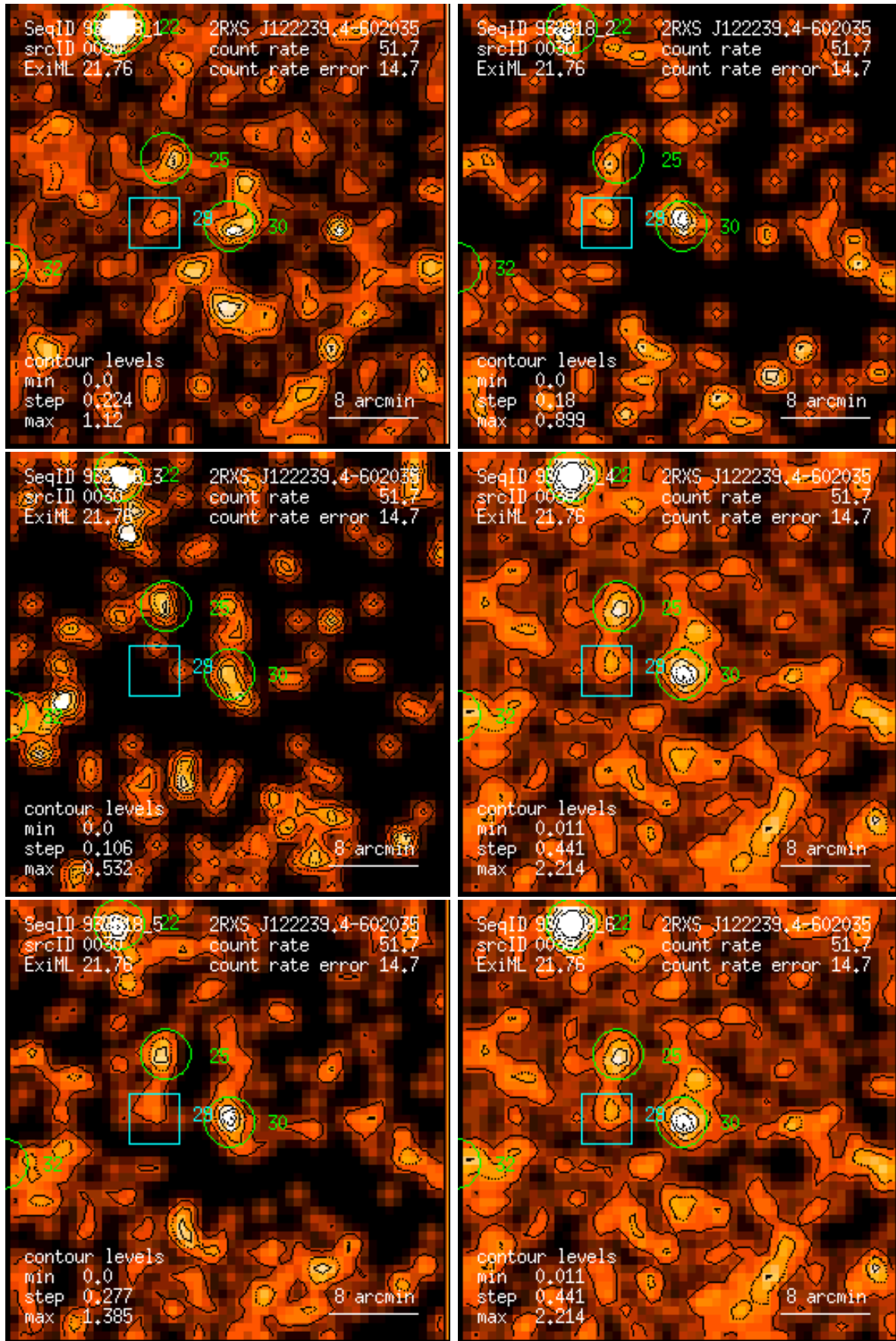
Figure 30: RASS 932818: detection 0030: band rate images, Gaussian filter: (1) PSPC channels 11 – 41, (2) 52 – 90, (3) 91 – 201, (4) 11 – 235, (5) 52 – 201, (6) 11 – 201. Broad band rates in counts/ks. Band rate contour levels in counts/ks/arcmin 2 .
