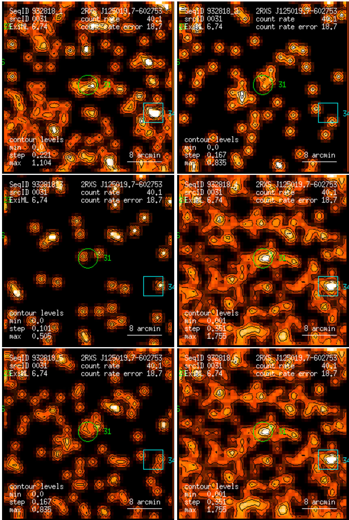
Figure 31: RASS 932818: detection 0031: band rate images, Gaussian filter: (1) PSPC channels 11 – 41, (2) 52 – 90, (3) 91 – 201, (4) 11 – 235, (5) 52 – 201, (6) 11 – 201. Broad band rates in counts/ks. Band rate contour levels in counts/ks/arcmin 2 .
