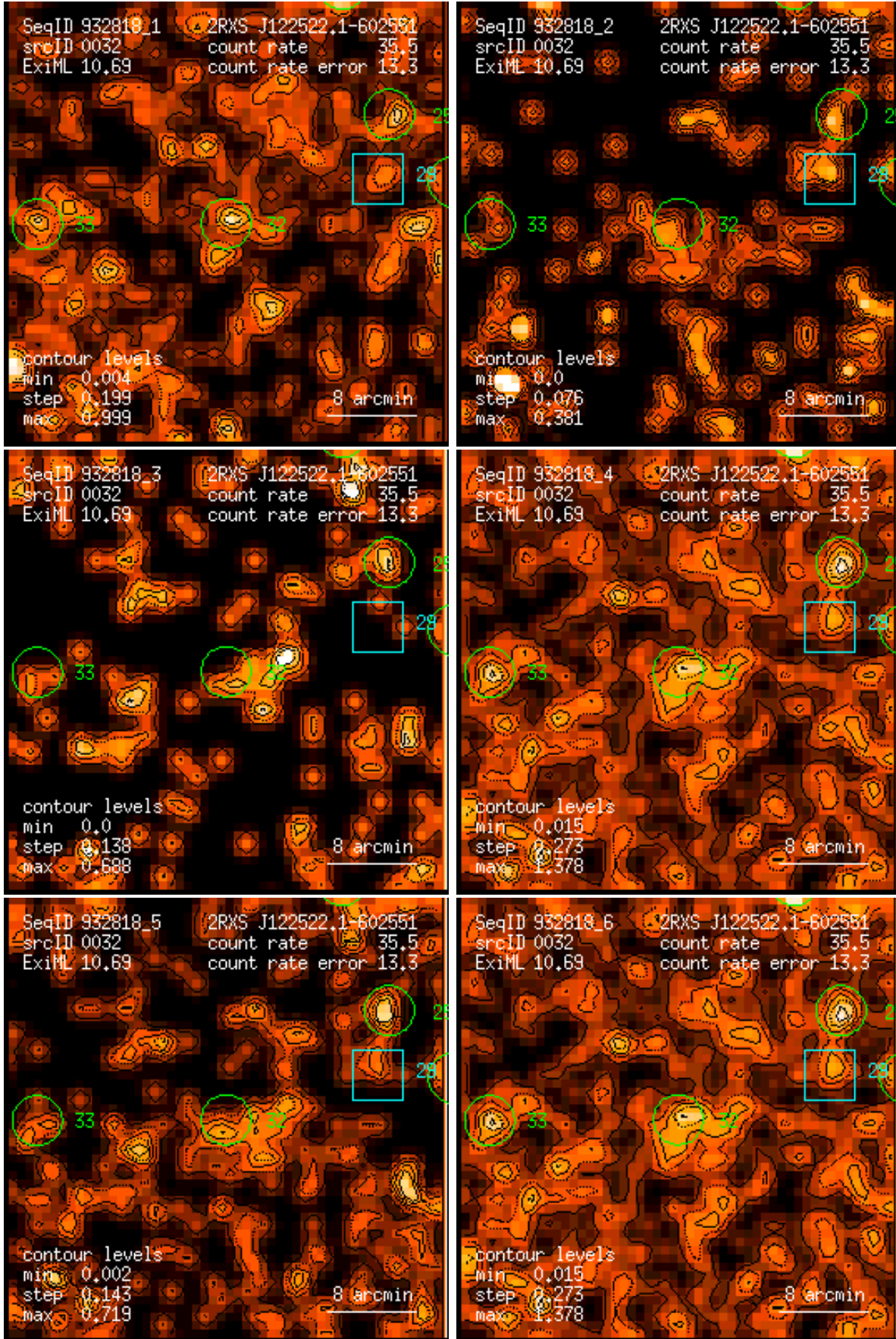
Figure 32: RASS 932818: detection 0032: band rate images, Gaussian filter: (1) PSPC channels 11 – 41, (2) 52 – 90, (3) 91 – 201, (4) 11 – 235, (5) 52 – 201, (6) 11 – 201. Broad band rates in counts/ks. Band rate contour levels in counts/ks/arcmin 2 .
