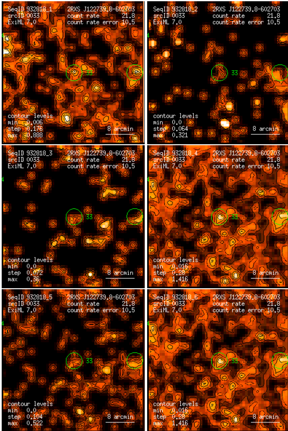
Figure 33: RASS 932818: detection 0033: band rate images, Gaussian filter: (1) PSPC channels 11 – 41, (2) 52 – 90, (3) 91 – 201, (4) 11 – 235, (5) 52 – 201, (6) 11 – 201. Broad band rates in counts/ks. Band rate contour levels in counts/ks/arcmin 2 .
