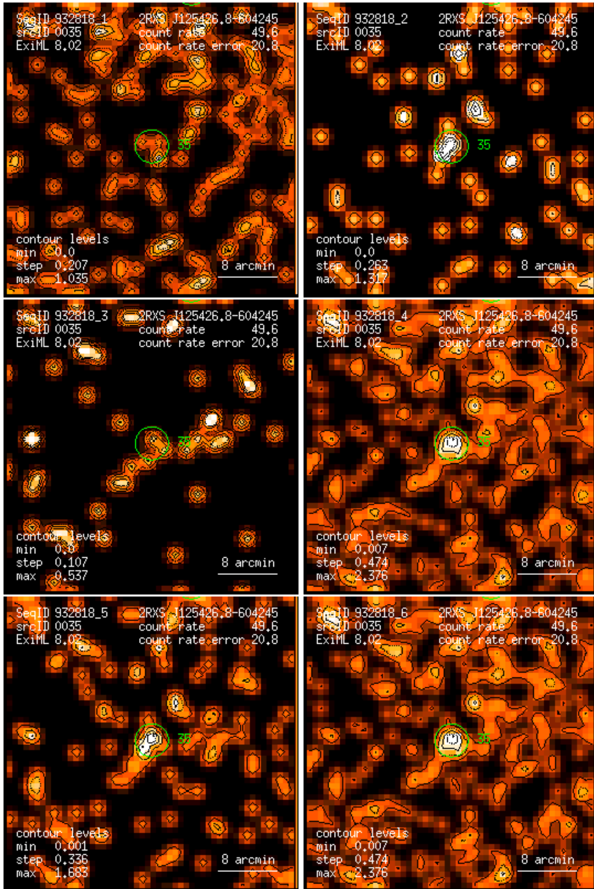
Figure 35: RASS 932818: detection 0035: band rate images, Gaussian filter: (1) PSPC channels 11 – 41, (2) 52 – 90, (3) 91 – 201, (4) 11 – 235, (5) 52 – 201, (6) 11 – 201. Broad band rates in counts/ks. Band rate contour levels in counts/ks/arcmin 2 .
