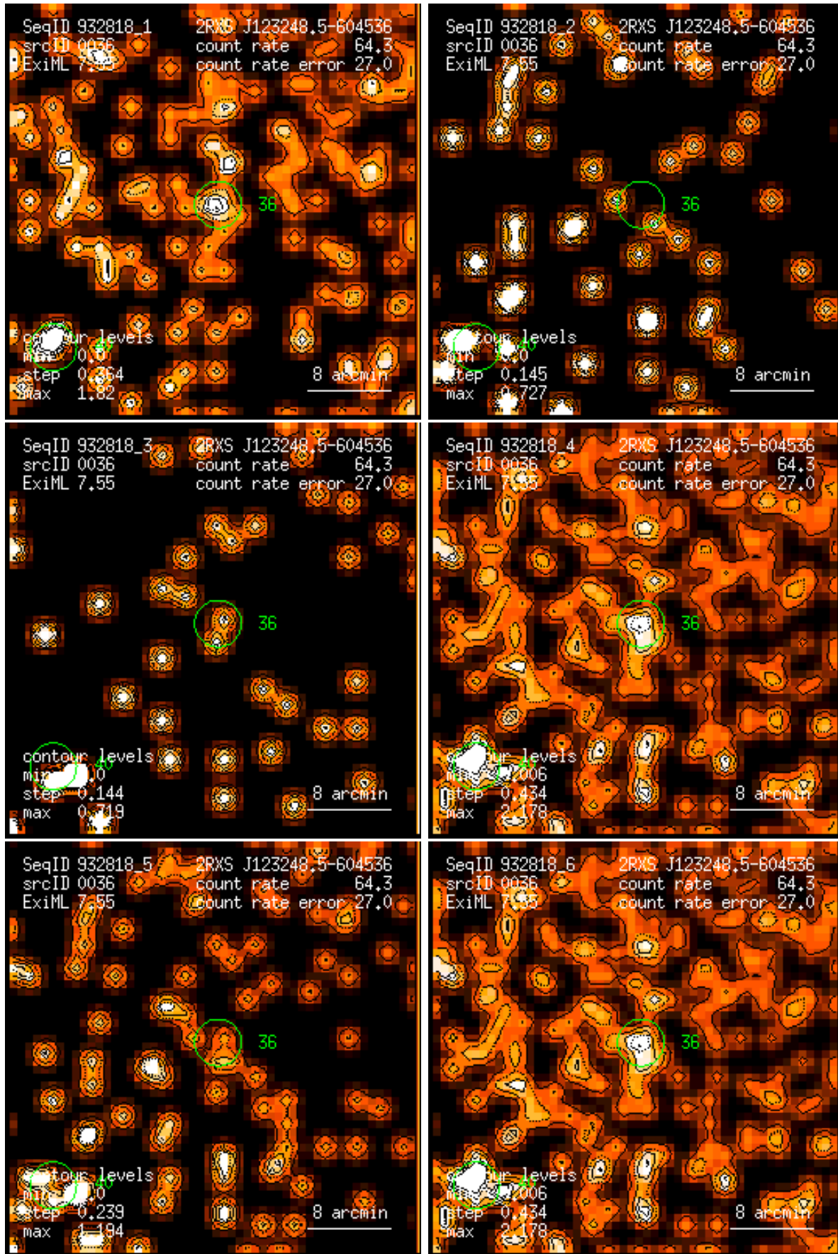
Figure 36: RASS 932818: detection 0036: band rate images, Gaussian filter: (1) PSPC channels 11 – 41, (2) 52 – 90, (3) 91 – 201, (4) 11 – 235, (5) 52 – 201, (6) 11 – 201. Broad band rates in counts/ks. Band rate contour levels in counts/ks/arcmin 2 .
