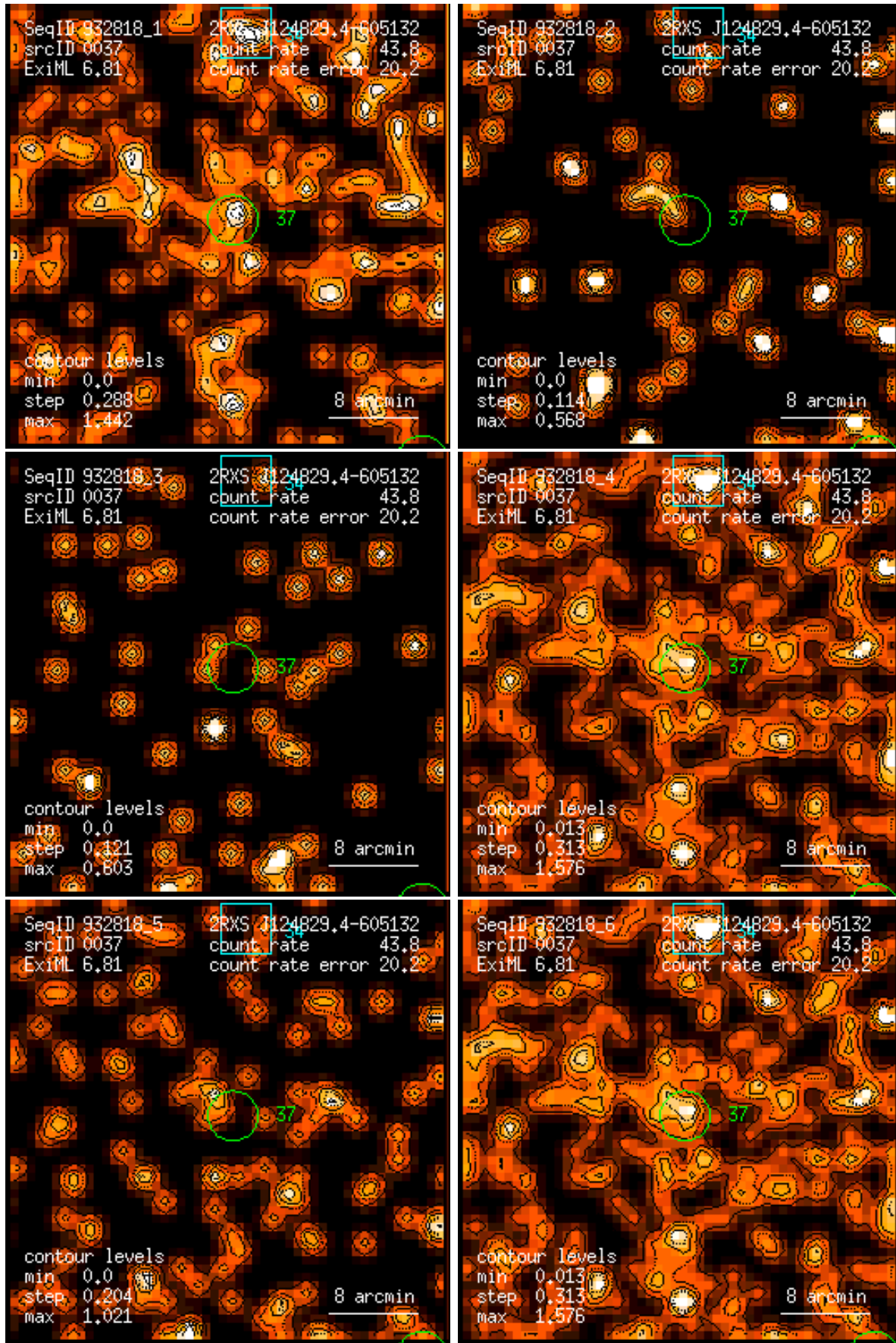
Figure 37: RASS 932818: detection 0037: band rate images, Gaussian filter: (1) PSPC channels 11 – 41, (2) 52 – 90, (3) 91 – 201, (4) 11 – 235, (5) 52 – 201, (6) 11 – 201. Broad band rates in counts/ks. Band rate contour levels in counts/ks/arcmin 2 .
