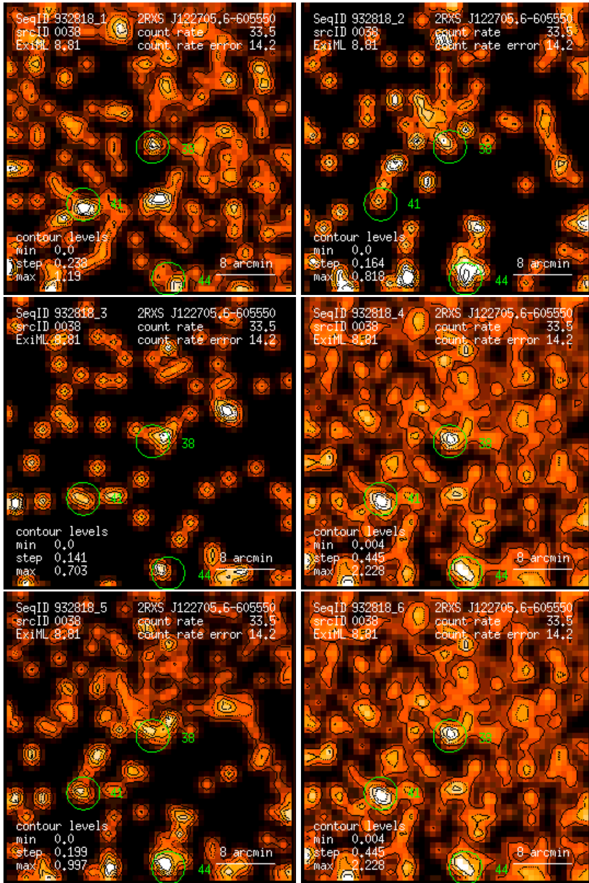
Figure 38: RASS 932818: detection 0038: band rate images, Gaussian filter: (1) PSPC channels 11 – 41, (2) 52 – 90, (3) 91 – 201, (4) 11 – 235, (5) 52 – 201, (6) 11 – 201. Broad band rates in counts/ks. Band rate contour levels in counts/ks/arcmin 2 .
