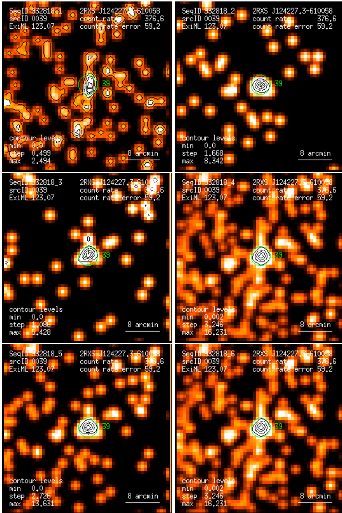
Figure 39: RASS 932818: detection 0039: band rate images, Gaussian filter: (1) PSPC channels 11 – 41, (2) 52 – 90, (3) 91 – 201, (4) 11 – 235, (5) 52 – 201, (6) 11 – 201. Broad band rates in counts/ks. Band rate contour levels in counts/ks/arcmin 2 .
