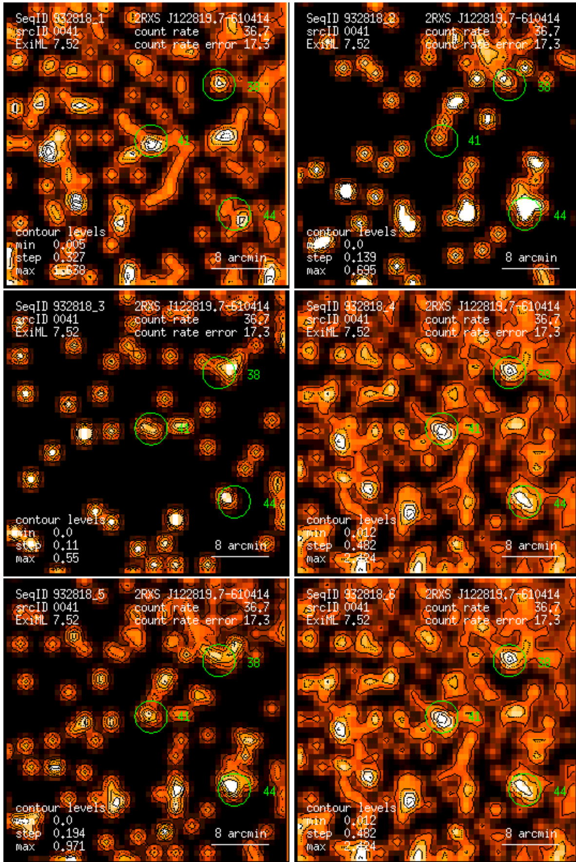
Figure 41: RASS 932818: detection 0041: band rate images, Gaussian filter: (1) PSPC channels 11 – 41, (2) 52 – 90, (3) 91 – 201, (4) 11 – 235, (5) 52 – 201, (6) 11 – 201. Broad band rates in counts/ks. Band rate contour levels in counts/ks/arcmin 2 .
