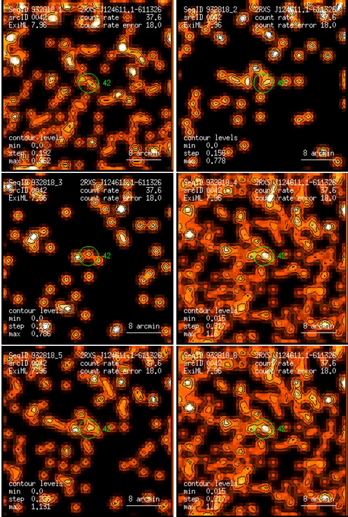
Figure 42: RASS 932818: detection 0042: band rate images, Gaussian filter: (1) PSPC channels 11 – 41, (2) 52 – 90, (3) 91 – 201, (4) 11 – 235, (5) 52 – 201, (6) 11 – 201. Broad band rates in counts/ks. Band rate contour levels in counts/ks/arcmin 2 .
