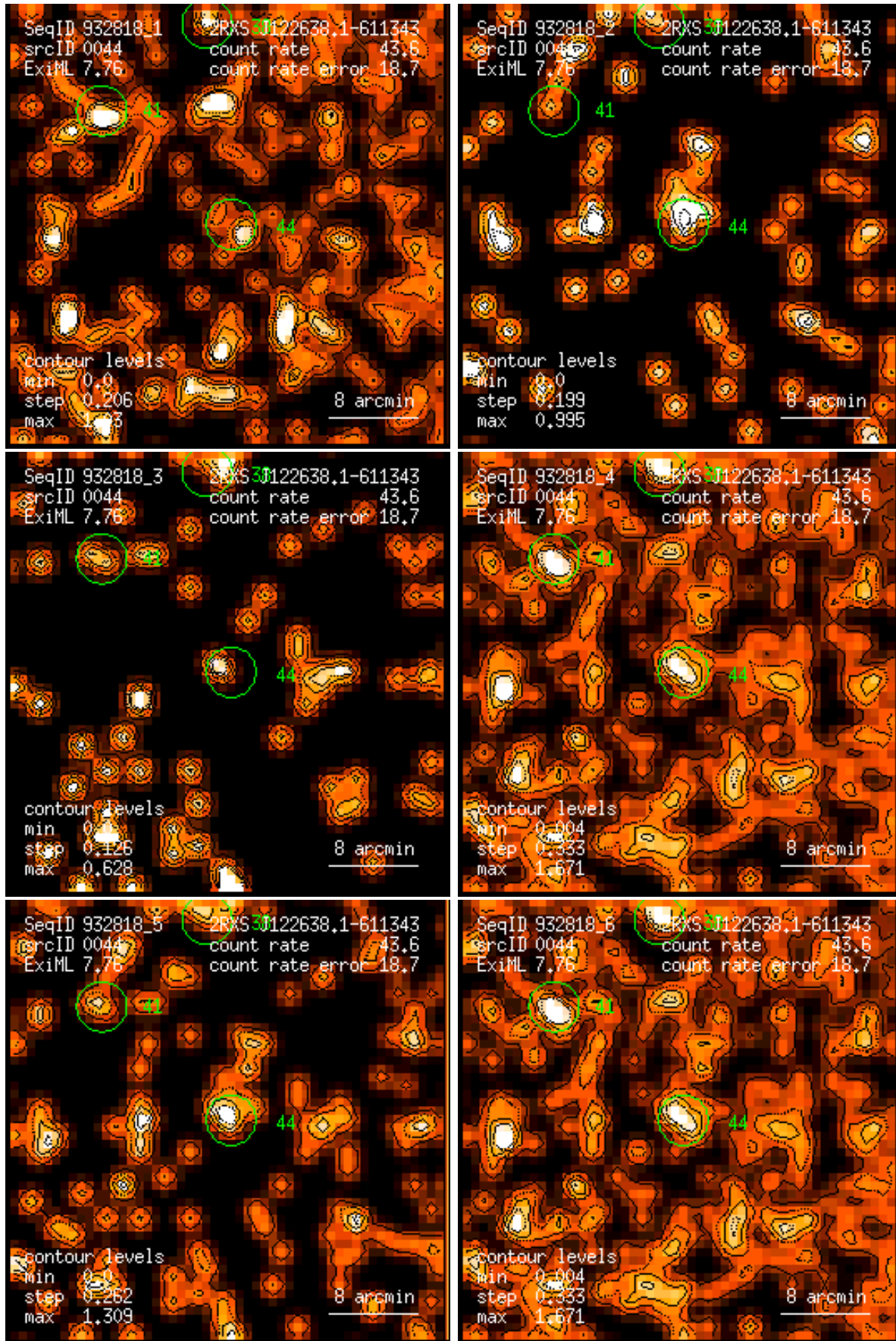
Figure 44: RASS 932818: detection 0044: band rate images, Gaussian filter: (1) PSPC channels 11 – 41, (2) 52 – 90, (3) 91 – 201, (4) 11 – 235, (5) 52 – 201, (6) 11 – 201. Broad band rates in counts/ks. Band rate contour levels in counts/ks/arcmin 2 .
