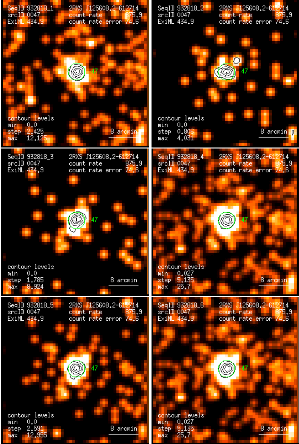
Figure 47: RASS 932818: detection 0047: band rate images, Gaussian filter: (1) PSPC channels 11 – 41, (2) 52 – 90, (3) 91 – 201, (4) 11 – 235, (5) 52 – 201, (6) 11 – 201. Broad band rates in counts/ks. Band rate contour levels in counts/ks/arcmin 2 .
