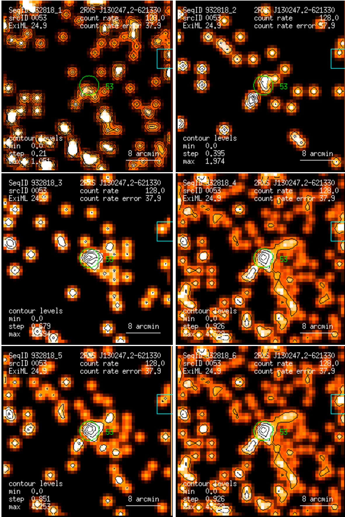
Figure 53: RASS 932818: detection 0053: band rate images, Gaussian filter: (1) PSPC channels 11 – 41, (2) 52 – 90, (3) 91 – 201, (4) 11 – 235, (5) 52 – 201, (6) 11 – 201. Broad band rates in counts/ks. Band rate contour levels in counts/ks/arcmin 2 .
